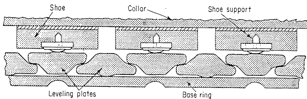
FIGURE 2-13B EQUALIZED SUPPORT OF THRUST BEARING SHOES
