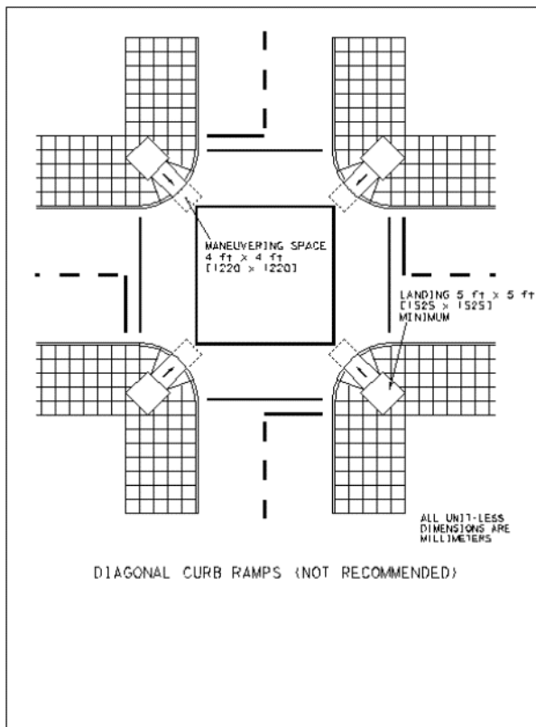
Figure 2-12. Diagonal Curb Ramps (Not Recommended). Click here to see a PDF of the image.
