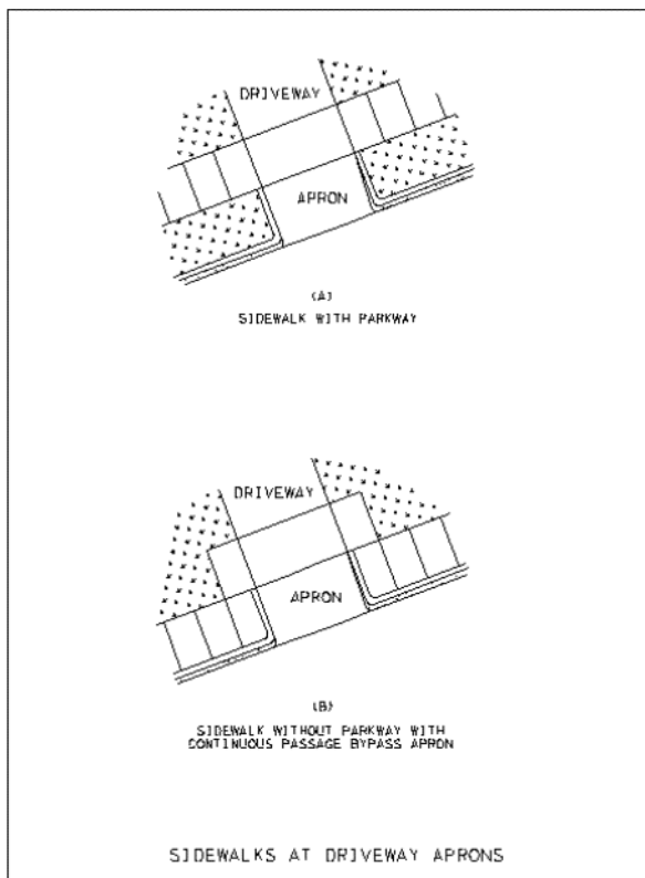
Figure 2-9. Sidewalks at Driveway Aprons. Click here to see a PDF of the image.
