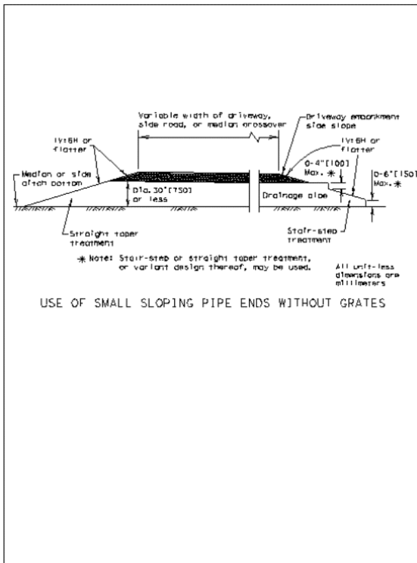
Figure 2-14. Use of Small Sloping Pipe Ends Without Grates. Click here to see a PDF of the image.
