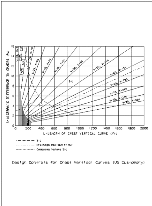
Figure 2-7. Design Controls for Crest Vertical Curves. Click US Customary or Metric to see a PDF of the image.
