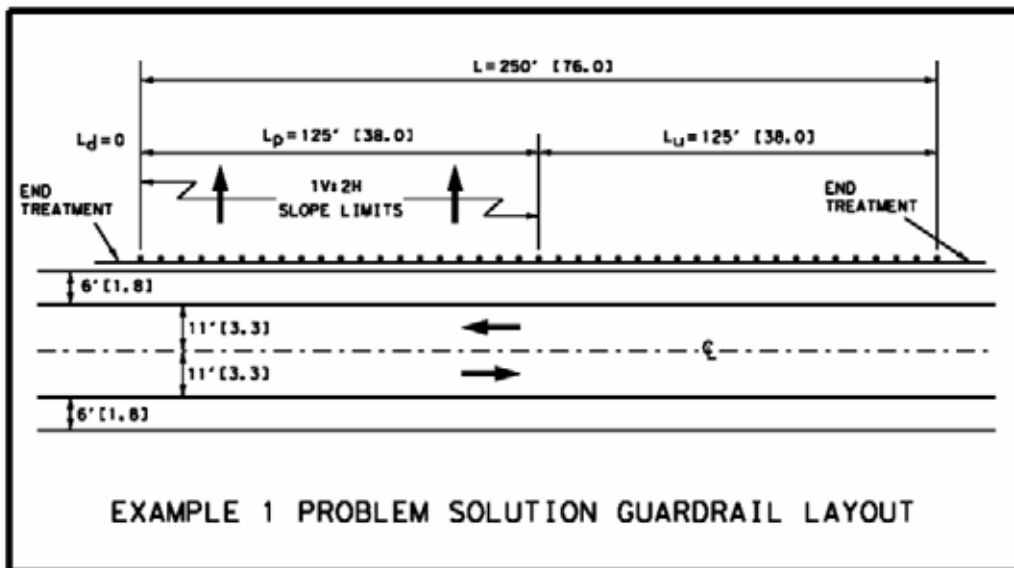
Figure A-10. Example 1 Problem Solution Guardrail Layout
