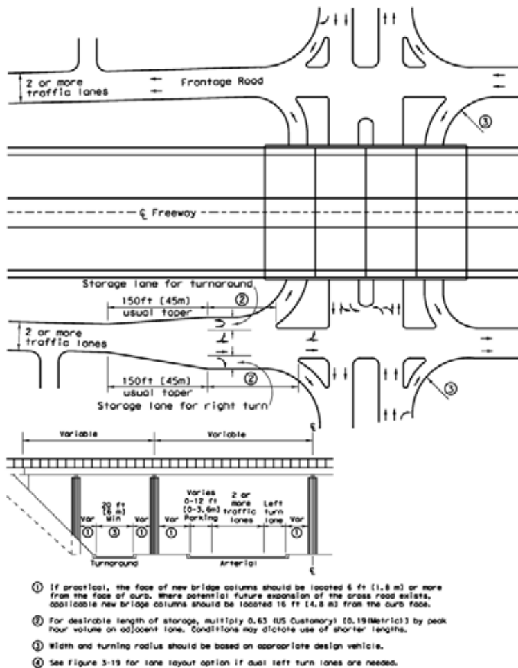
TYPICAL DIAMOND INTERCHANGE WITH FRONTAGE ROAD
