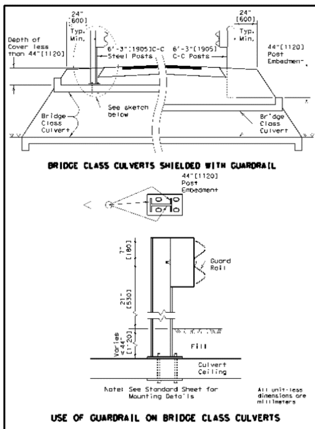
Figure 2-13. Use of Guardrail on Bridge Class Culverts. Click here to see a PDF of the image.
