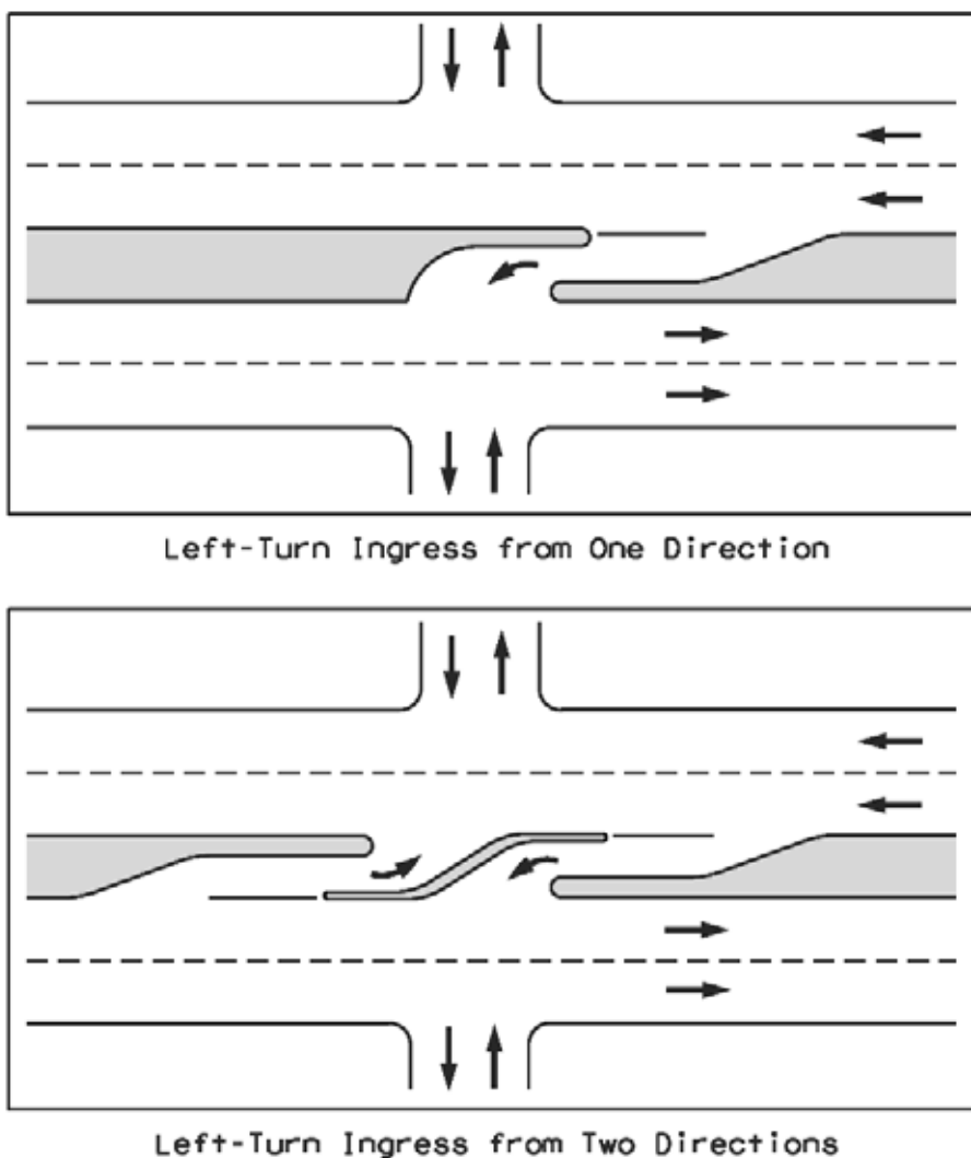
Figure 3-1. Types of Directional Openings. Click here to see a PDF of the image.
