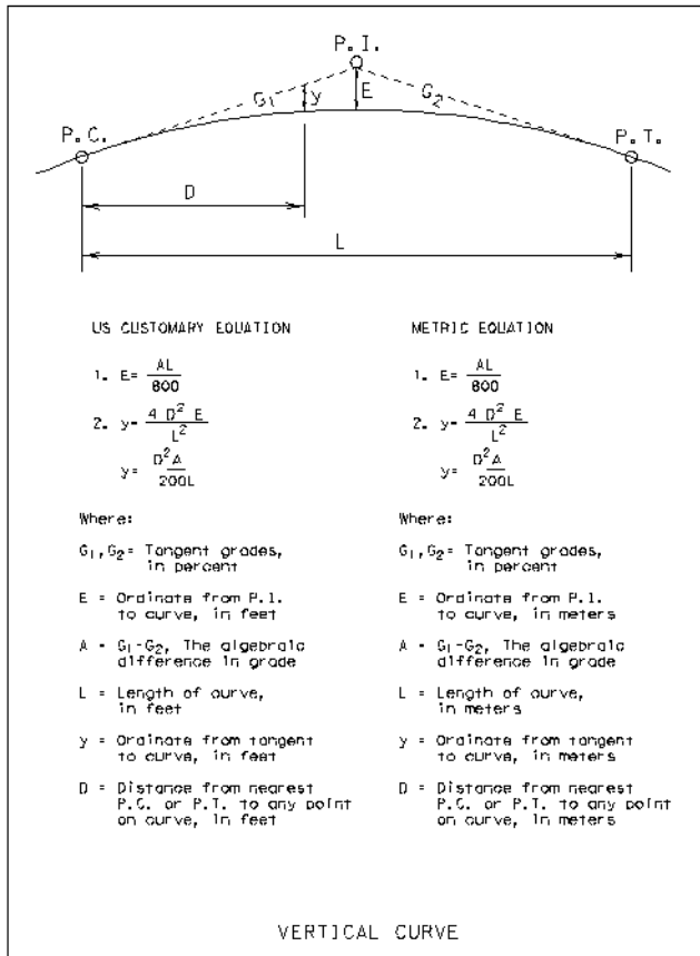
Figure 2-6. Vertical Curve. Click here to see a PDF of the image.
