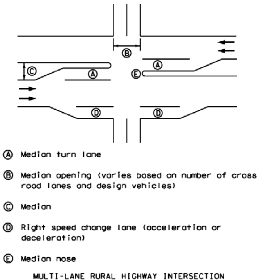
Figure 3-9. Multi-Lane Rural Highway Intersection. Click here to see a PDF of the image.
