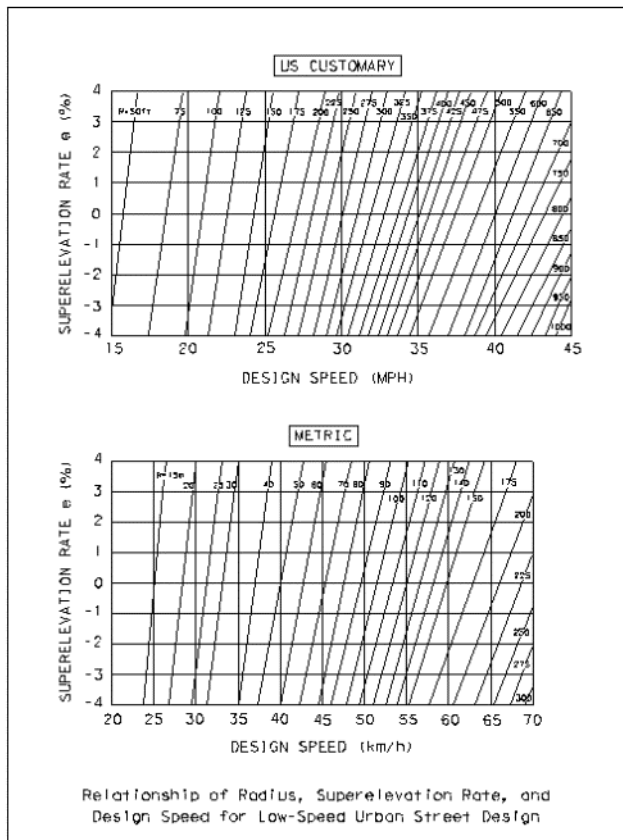
Figure 2-2. Relationship of Radius, Superelevation Rate, and Design Speed for Low-Speed Urban Street Design. Click here to see a PDF of the image.
