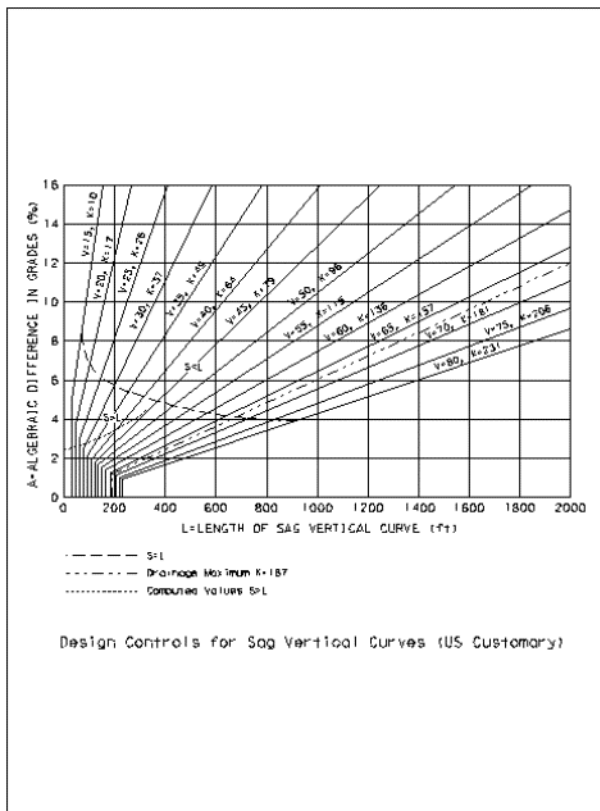
Figure 2-8. (US). Design Controls for Sag Vertical Curves. Click US Customary or Metric to see a PDF of this image.
