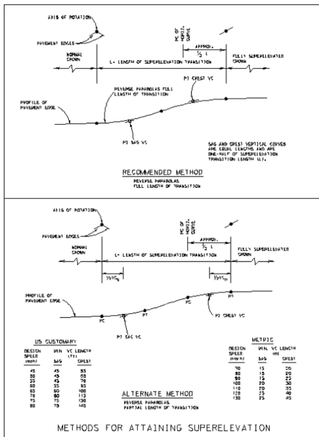
Figure 2-1. Methods for Attaining Superelevation. Click here to see a PDF of the image.
