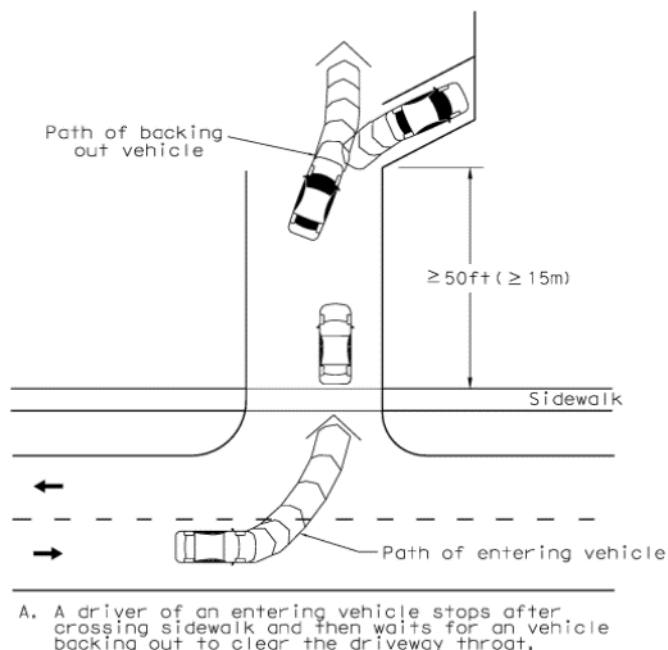
Figure C-13. Throat Length is of Sufficient Length to Allow Entering Vehicle to Clear the Through Traffic Lane
