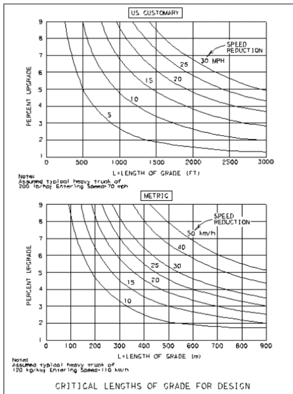
Figure 2-5. Critical Lengths of Grade for Design. Click here to see a PDF of this image.
