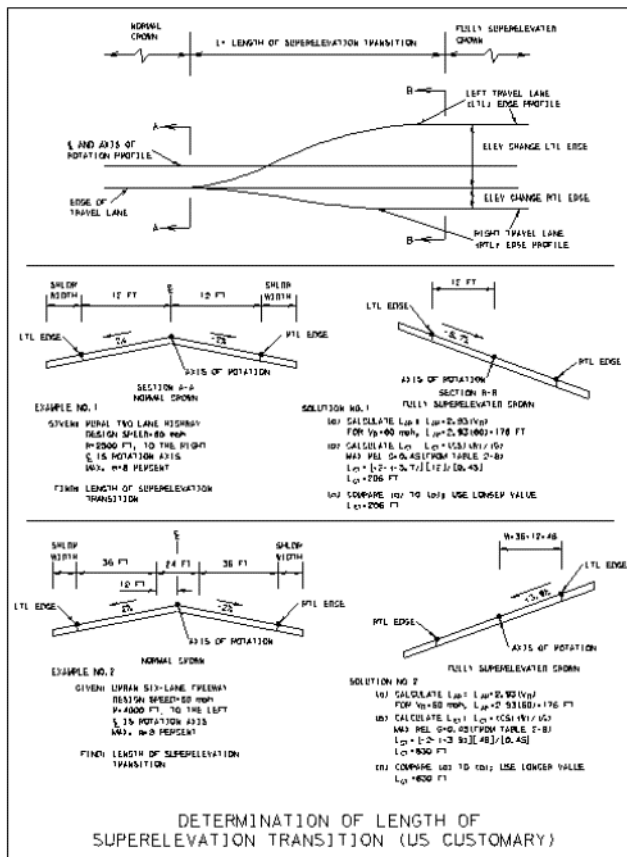
Figure 2-3. Determination of Length of Superelevation Transition. Click US Customary or Metric to see a PDF of the image.
