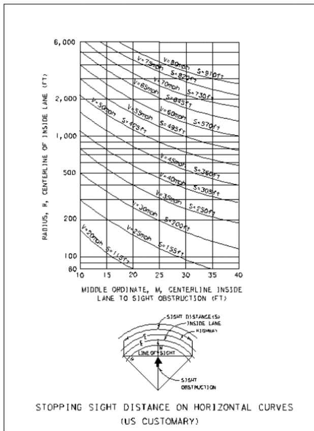
Figure 2-4. (US). Stopping Sight Distance on Horizontal Curves. Click US Customary or Metric to see a PDF of the image.
