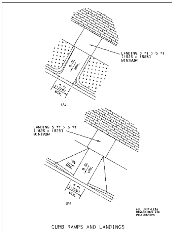
Figure 2-10. Curb Ramps and Landings. Click here to see a PDF of the image.
