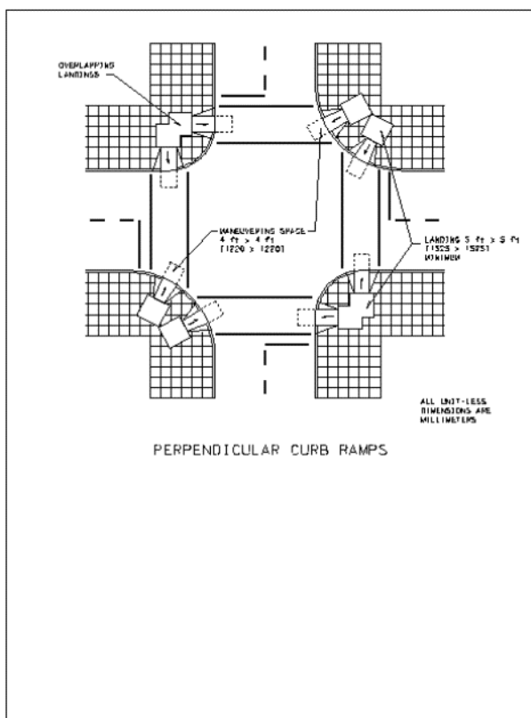
Figure 2-11. Perpendicular Curb Ramps. Click here to see a PDF of the image.
