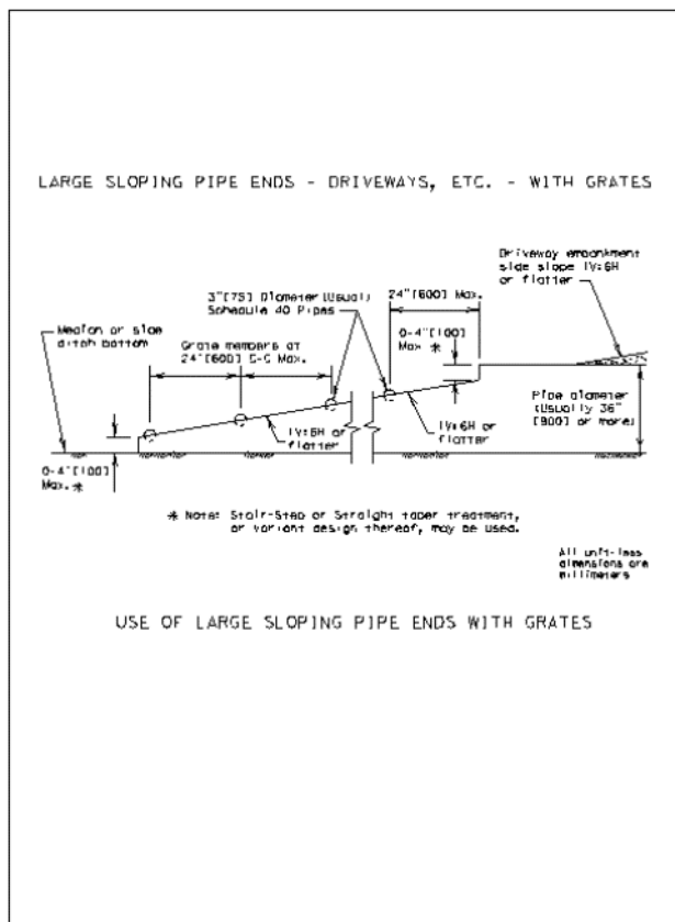
Figure 2-15. Use of Large Sloping Pipe Ends With Grates. Click here to see a PDF of the image.
