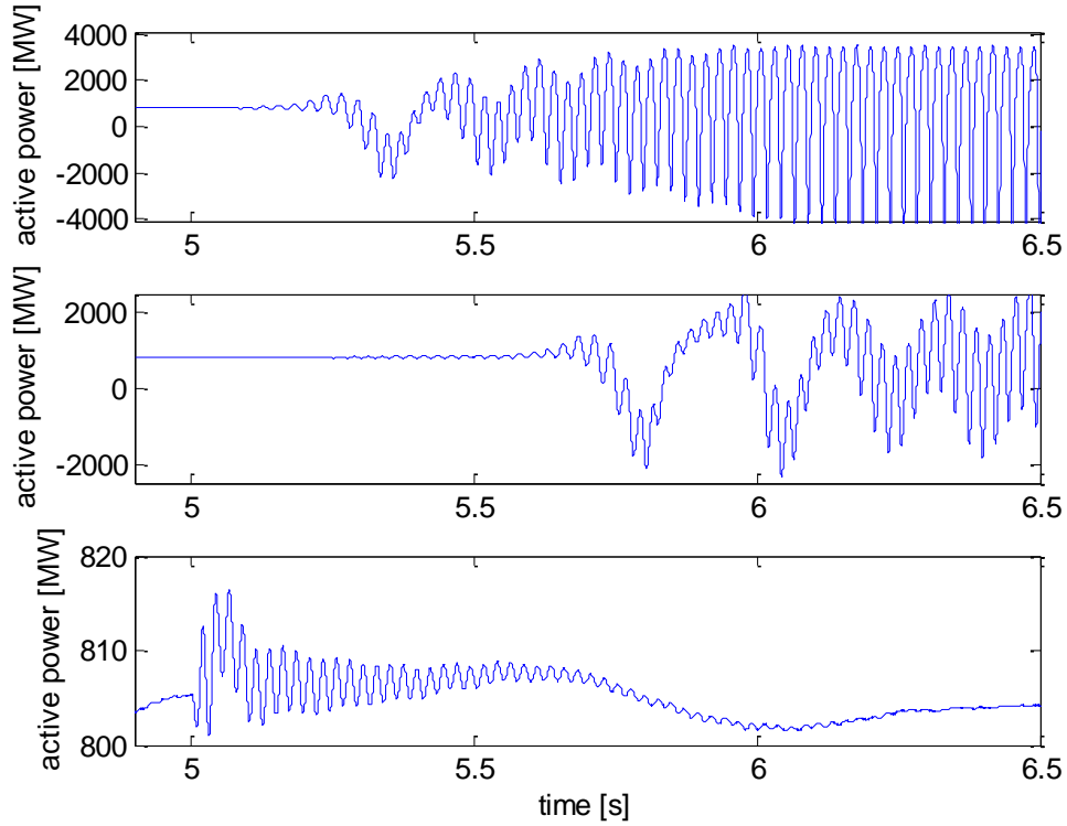
Fig. 32 - Transmitted active power after line disconnection. Series compensation level equal to 68%. Top: 2 pu, ideal dc source case; middle: 4 pu, ideal dc source case; bottom: 10 pu, actual configuration. Output power equal to 0.9pu.
