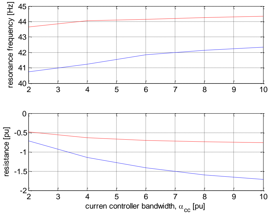
Fig. 28 - Trend of DFIG resonance frequency (top) and corresponding equivalent resistance (bottom) as a function of the current controller bandwidth. Comparison between ideal dc source case (blue curve) and actual configuration (red curve). Output power equal to 0.9pu.
