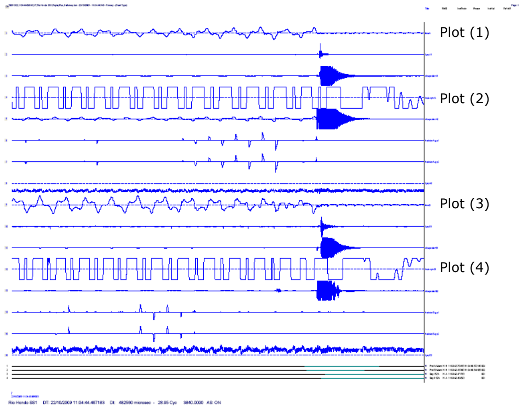
Fig. 11 - Measured quantities at the Rio Hondo series-capacitor banks. Plot (1): line current in phase a ; Plot (2): subsynchronous current in phase a ; Plot (3): line current in phase b ; Plot (4) subsynchronous current in phase b . Additional measurements from the series-capacitor banks are also displayed in the figure.
