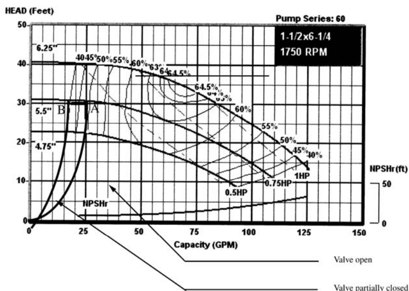
Fig 10-26. Pump curve for Series 60 B&amp;G inline pump
