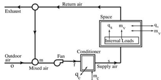
Fig 3-14. Air conditioning system
