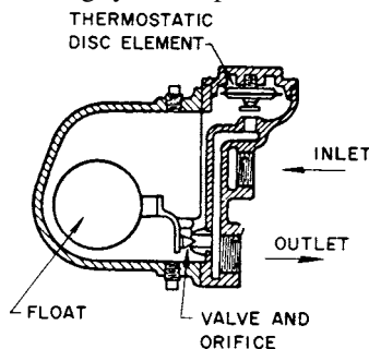
Fig 15-75. Typical float and thermostatic trap
