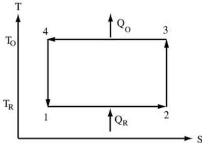
Fig 1-3. Carnot cycle
