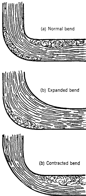
Fig 16-38. Air pattern in bends of various patterns
