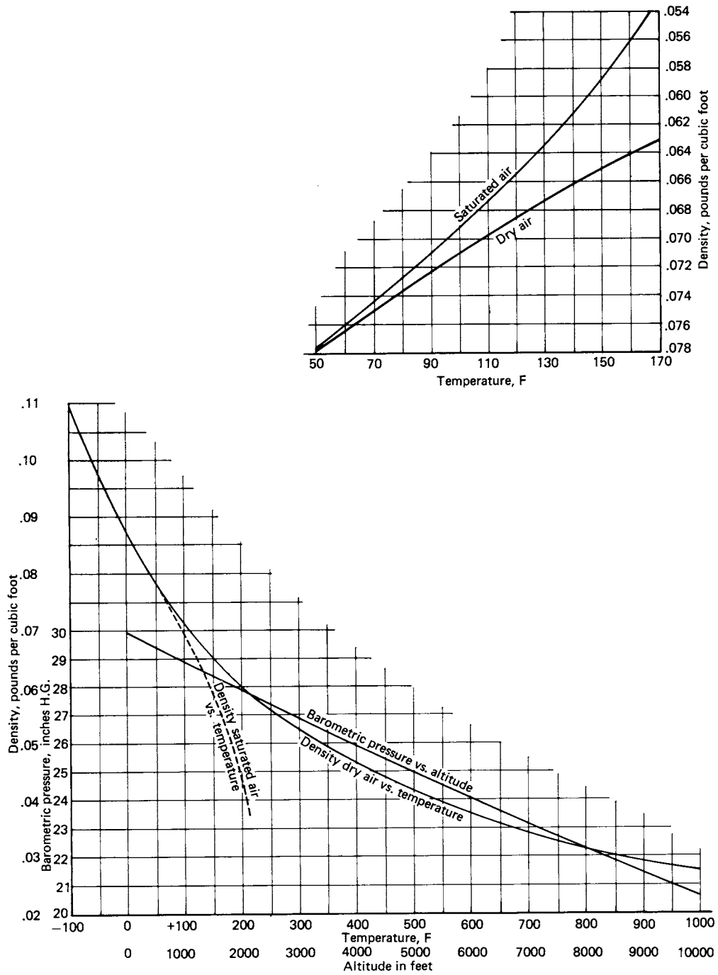
Fig 14-21. Density versus temperature and pressure versus elevation
