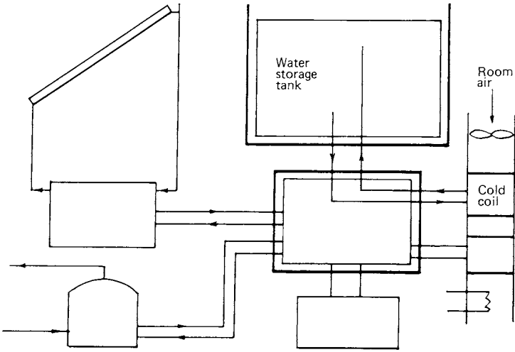
Fig 13-86. Utility off-peak space cooling
