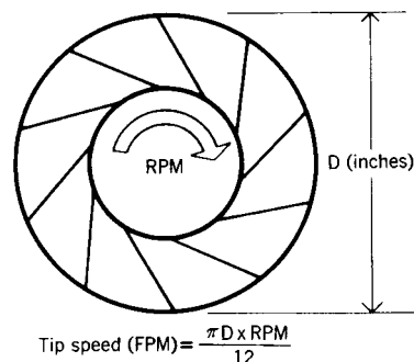
Fig 14-8. Tip speed
