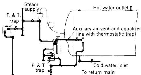
Fig 15-15. Piping connections to hot water generator
