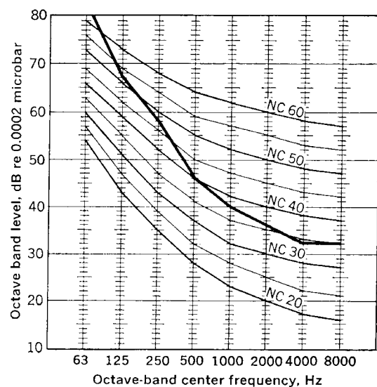
Fig 16-32. Typical curve of high velocity air distribution system generated noise
