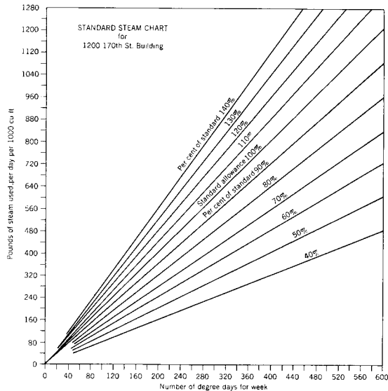
Fig 11-2. Example of chart prepared for a specific building to check operating efficiency
