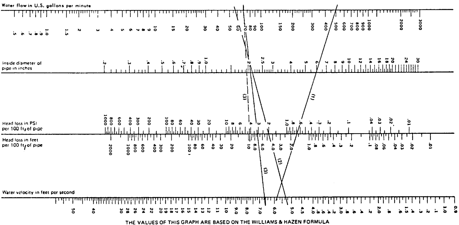
Fig 9-40. Flow loss characteristics of water flow through rigid plastic pipe
