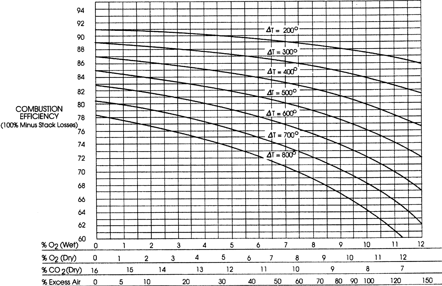
Fig 12-7, Combustion efficiency of No. 6 oil
