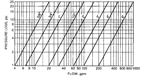
Fig 9-8. Pressure loss in disk type water meters
