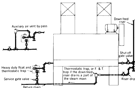
Fig 15-12. Piping connection for industrial type unit heater
