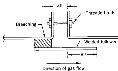
Fig 14-85. Expansion joint
