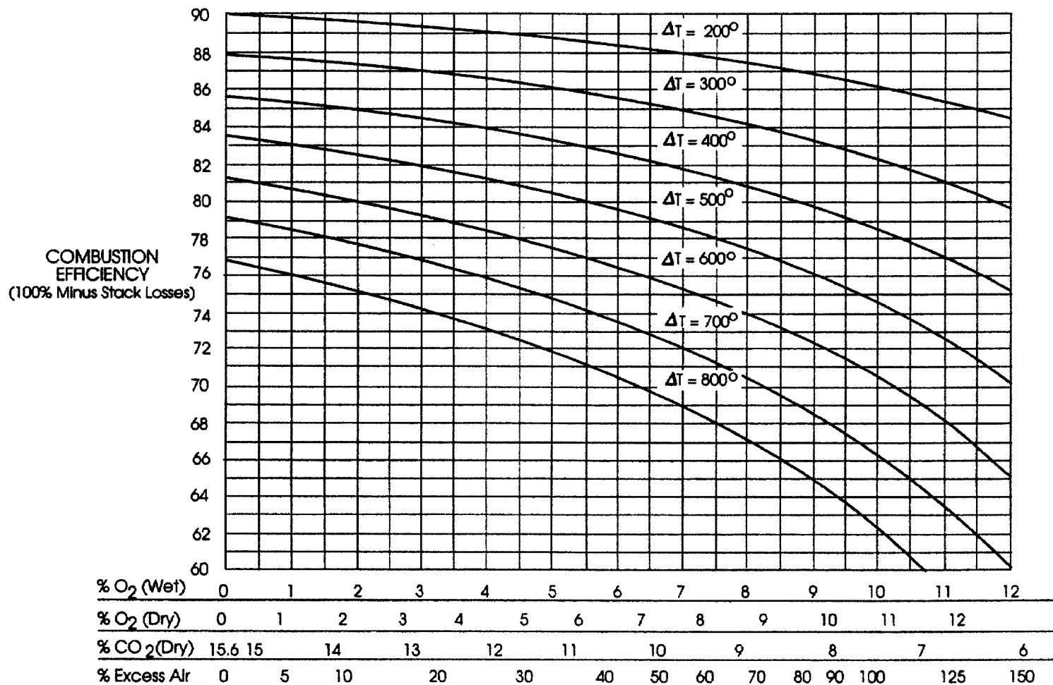
Fig 12-6. Combustion efficiency of No. 2 oil
