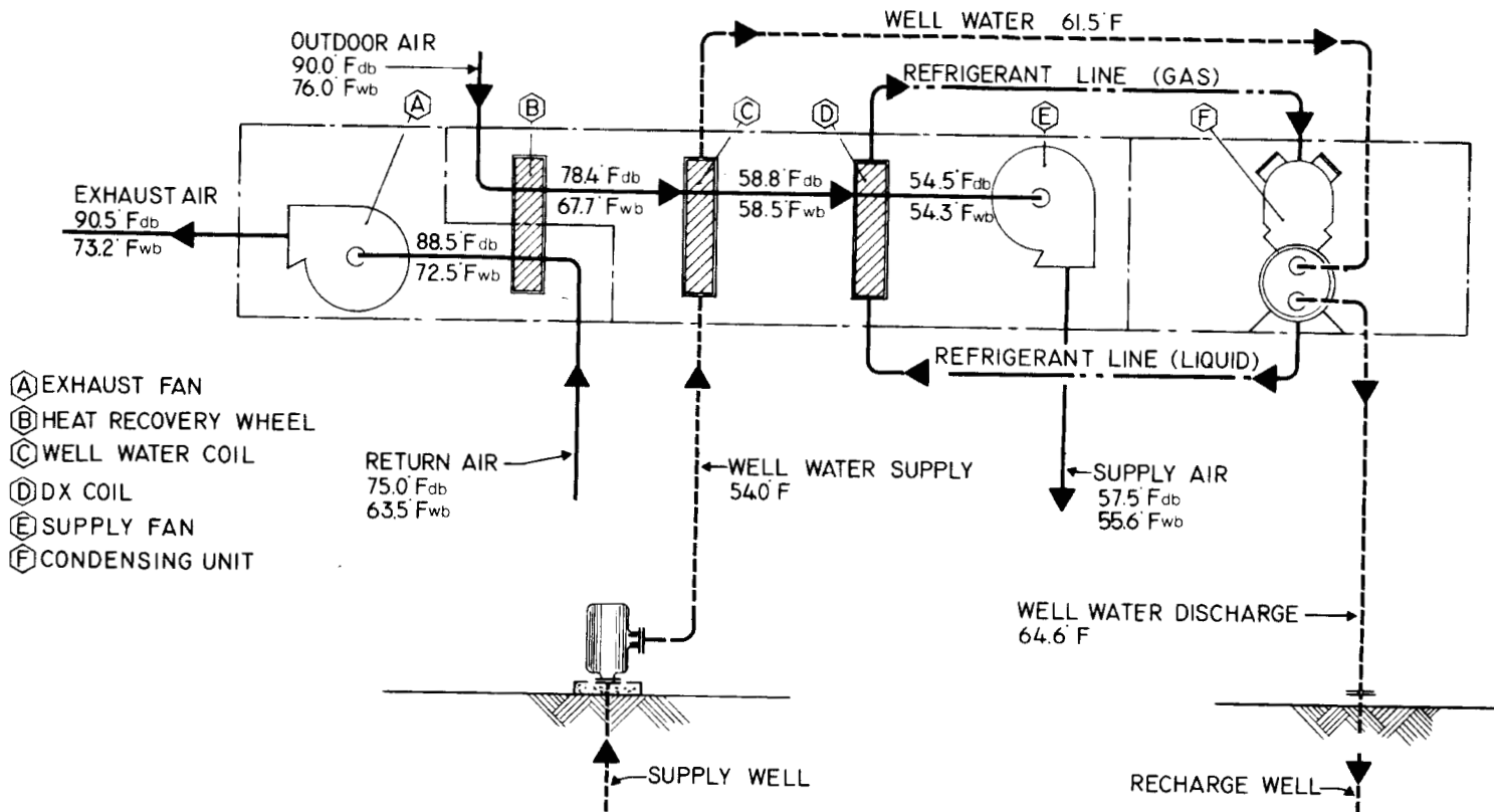
Fig 13-78. Schematic of well water precooling and refrigerant condensing system
