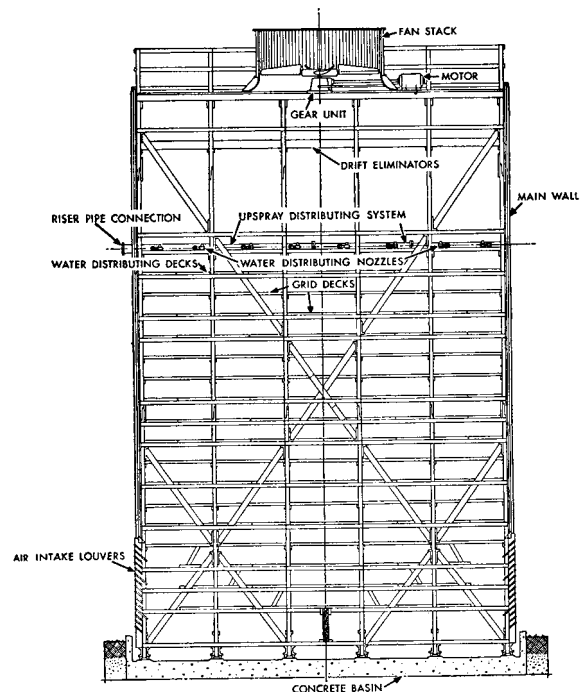
Fig 13-146. Cross section of mechanical draft cooling tower
