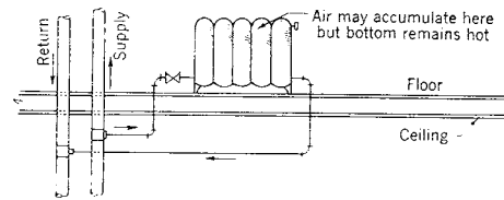
Fig 15-101. Preferred connection when radiation is above supply and return
