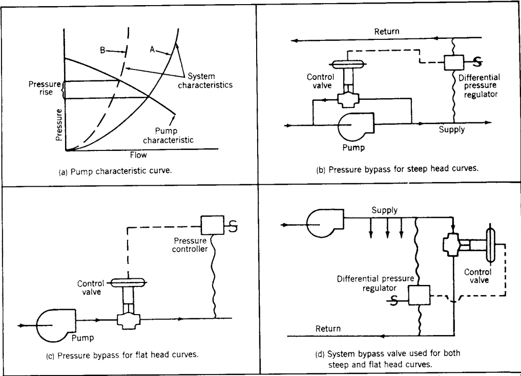
Fig 13-135. Hot water pressure control
