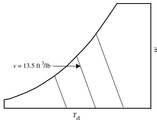
Fig 2-4c. Lines of constant specific volume v on the psychrometric chart
