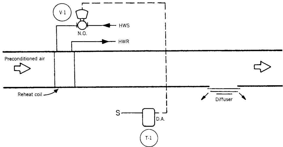
Fig 13-136. Hot water reheat control
