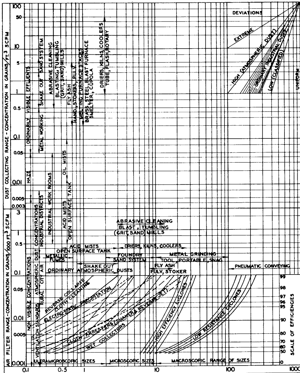
Fig 14-79. Range of particle sizes concentration and collector performance
