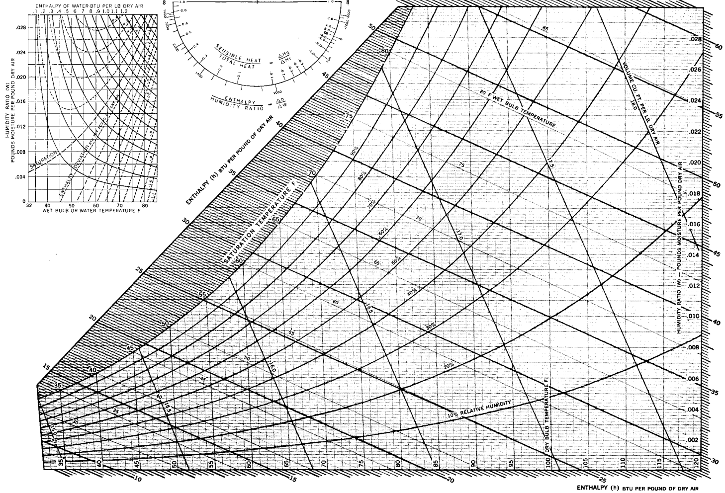
Fig 2-6. ASHRAE psychrometric chart (5000 ft)
