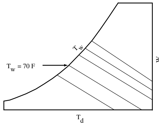
Fig 2-4d. Lines of constant wet bulb temperature T_w on the psychrometric chart
