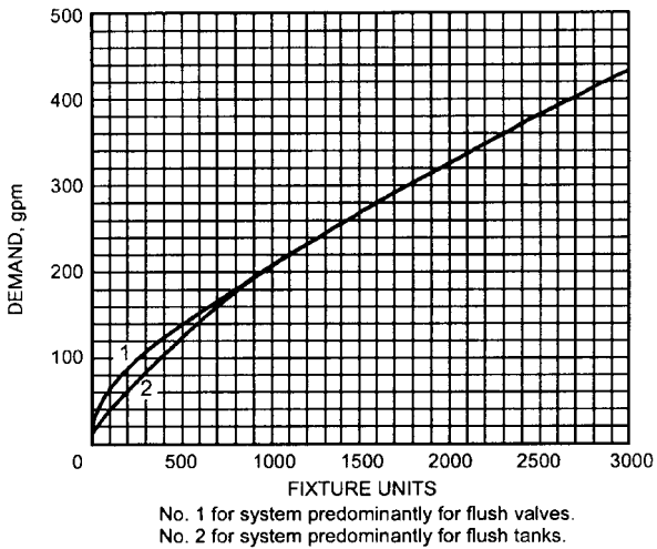
Fig 9-6. Estimate curves for demand load
