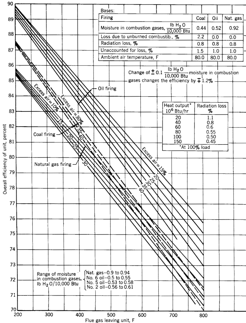
Fig 14-80. Overall efficiency of steam generating unit
