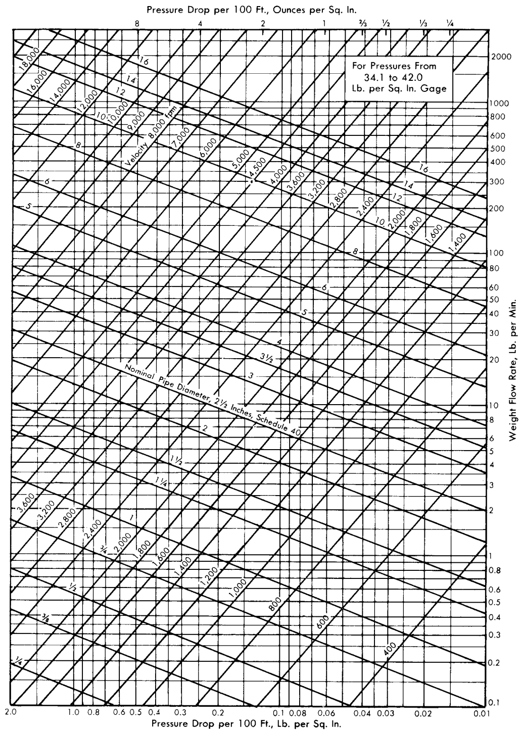
Fig 9-23. For pressure from 34.1 to 42.0 psig
