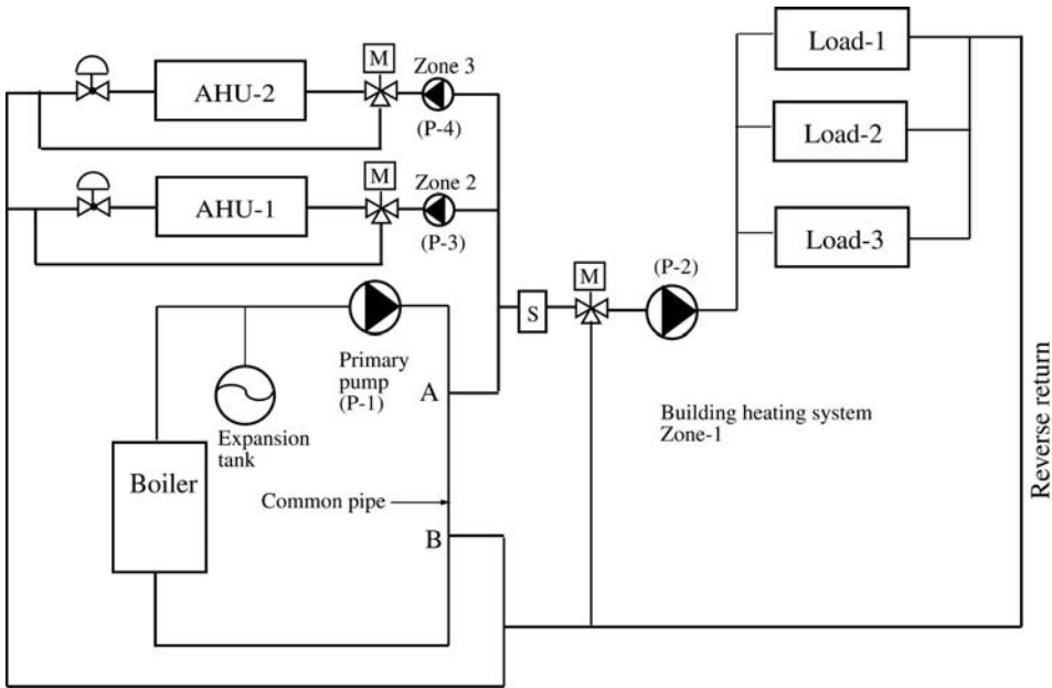
Fig 10-2. Heating system for multiple dwelling building with reverse return system
