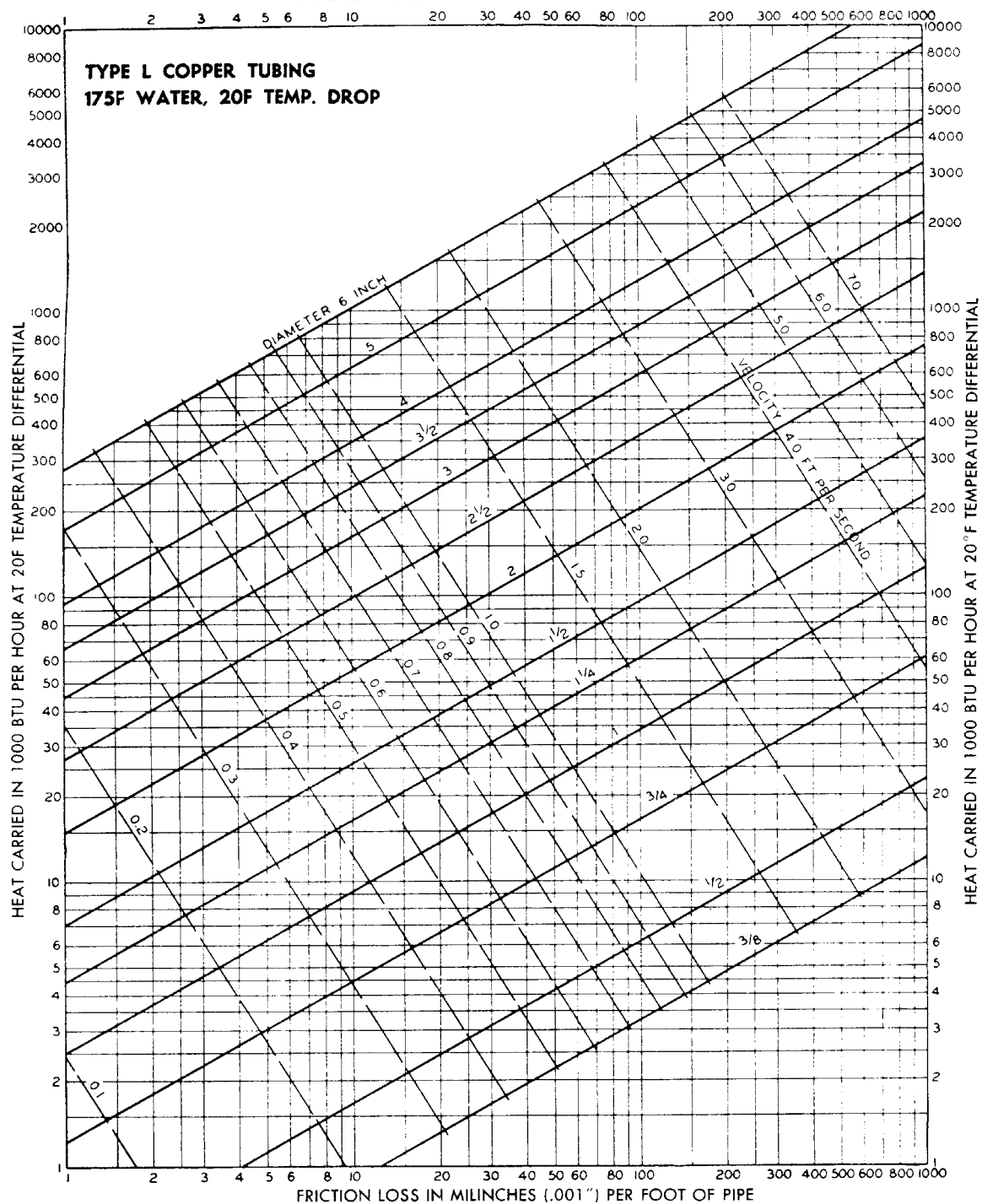
Fig 15-89. Hot water friction chart (for copper tube)
