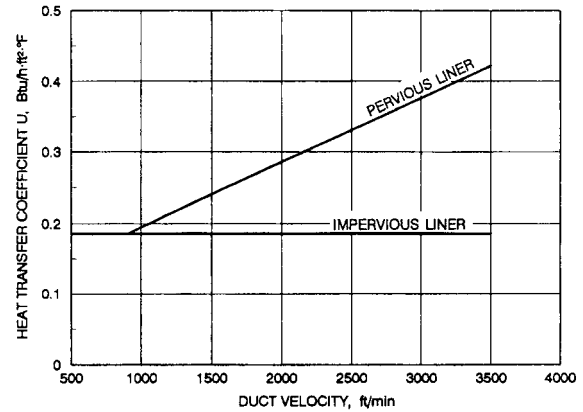
Fig 8-4b. Insulated flexible ducts
