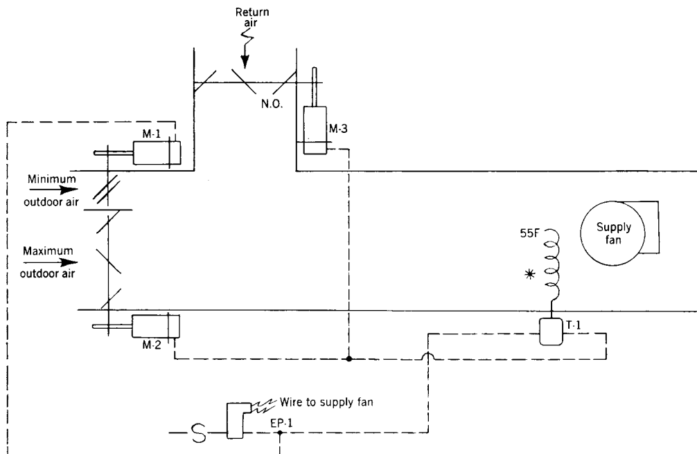
Fig 13-128. Changeover control
