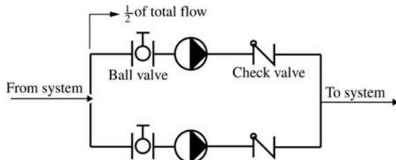
Fig 10-27. Typical installation of two pumps in parallel, with check valve
