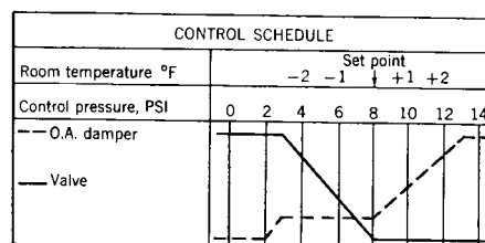
Fig 13-130. One day night operation
