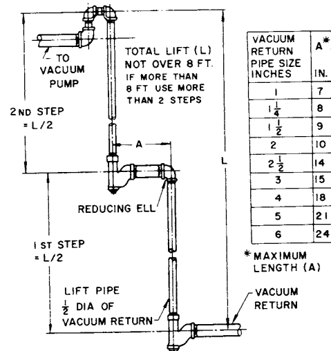
Fig 15-47. Two step condensate lift
