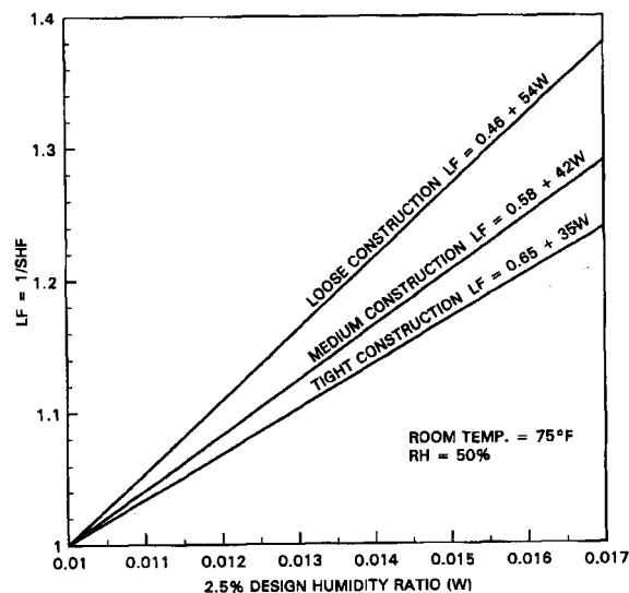
Fig 7-4. Effect of infiltration on latent load factor
