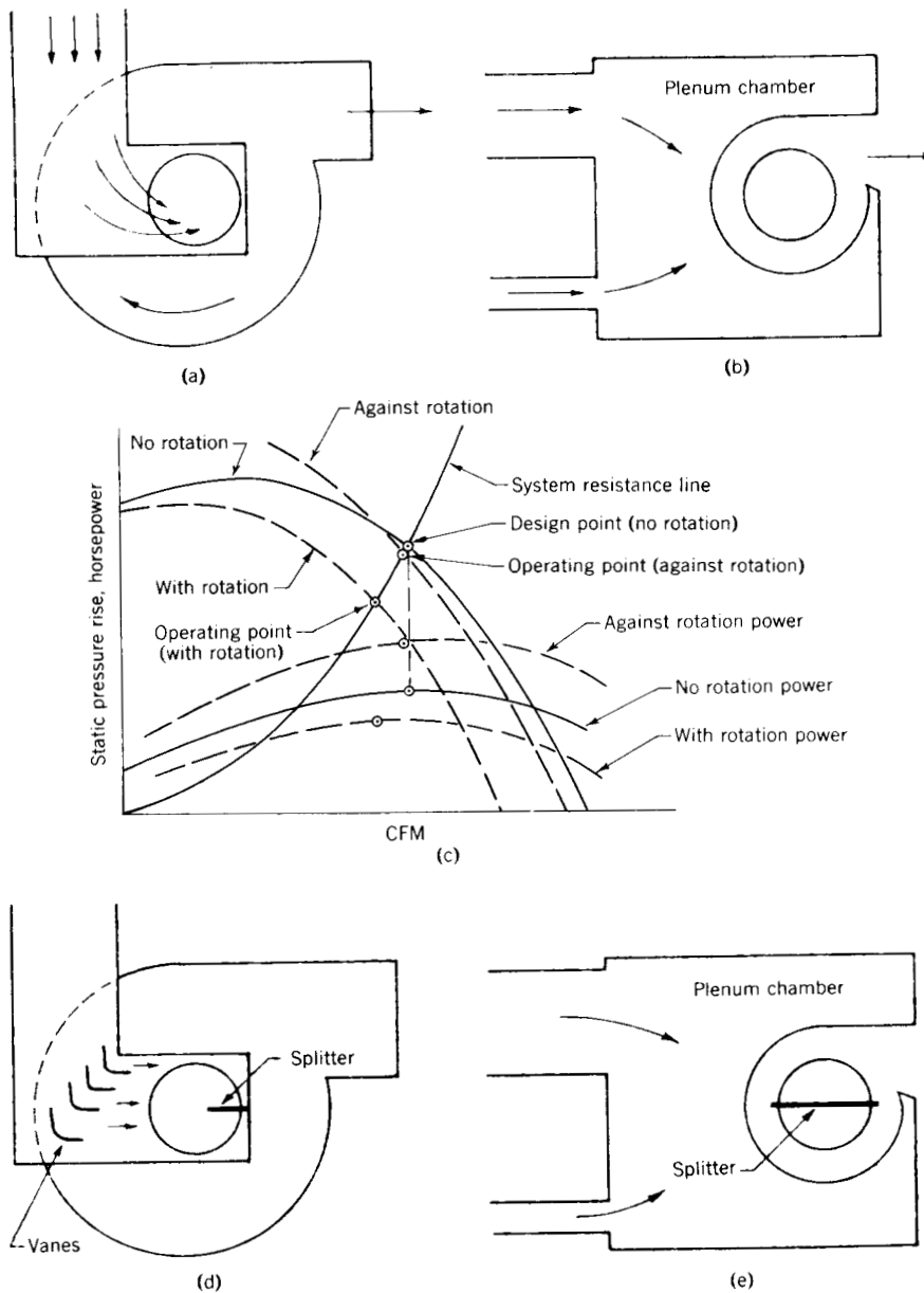
Fig 14-46. Fan inlet swirl (a) inertia of air tends to crowd it to bottom of inlet, setting up swirl. (b) with two unequally sized inlets to plenum chamber, imbalance is set-up, causing swirl at fan inlet. (c) effect of two-inlet swirl on fan performance. (d) vanes and splitter prevent swirl in inlet box. (e) a splitter overcomes the imbalance that is due to unequal inlets.
