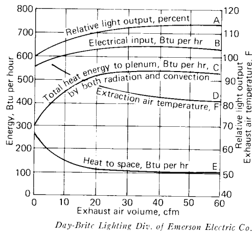
Fig 13-54. Manufacturer's data on heat distribution for a typical four lamp troffer
