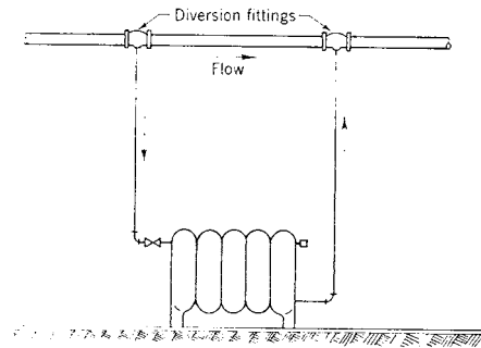
Fig 15-102. Preferred connection when radiation is below supply and return
