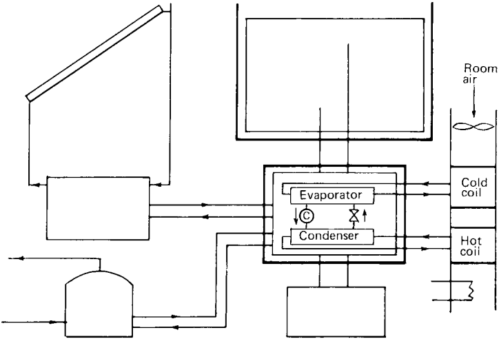
Fig 13-87. Dehumidification
