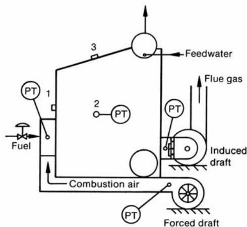
Fig 12-16. Measurement of furnace draft
