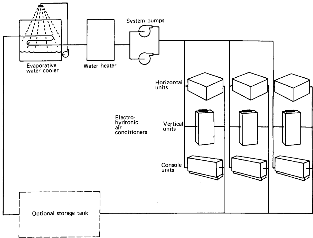
Fig 13-75. System water is cooled by evaporation of spray water, which is recirculated over the outside of the coil
