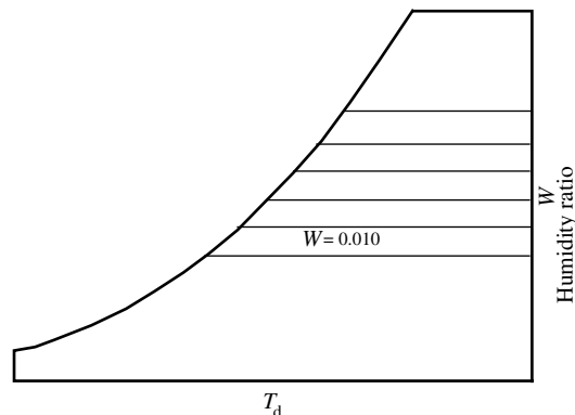
Fig 2-4b. Lines of constant humidity ratio ( W )
