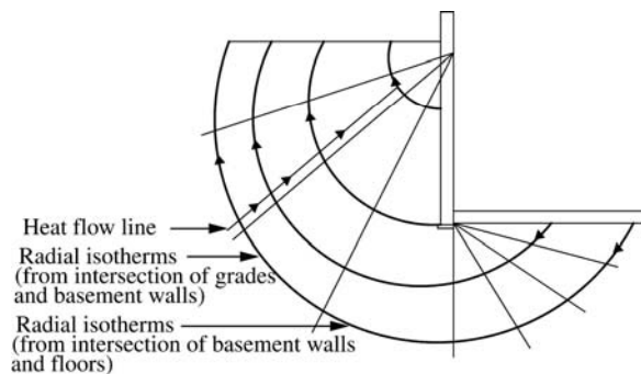
Fig 6-1. Heat flow from basement
