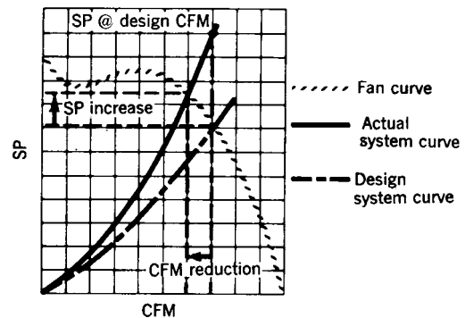
Fig 14-24. Variations from design—air shortage
