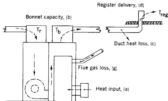
Fig 15-125. Furnace performance terminology
