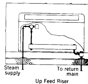
Fig 15-9. Convactor piping connection
