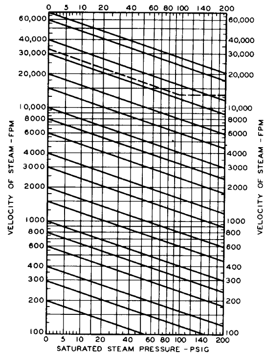
Fig 15-67. Velocity conversion
