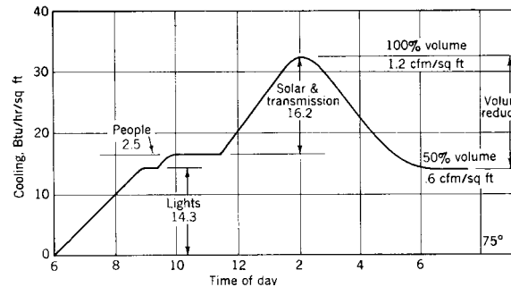
Fig 13-43. Load profile
