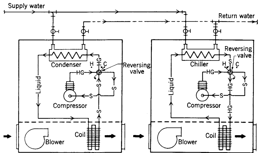
Fig 13-74. Water is recirculated in a loop as a heat reservoir
