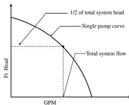
Fig 10-37. Basic series operation single pump curve
