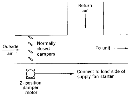
Fig 13-34. Simplest ventilation system
