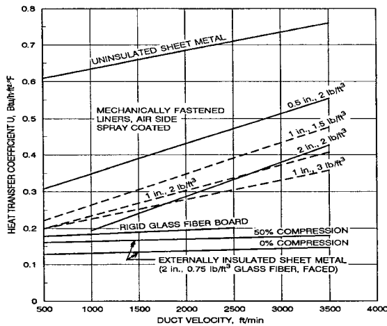
Fig 8-4a. Rigid ducts
