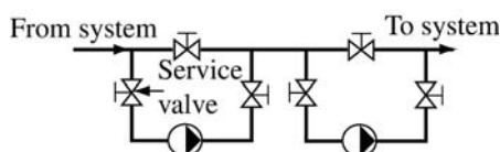
Fig 10-36. Practical series pump installation
