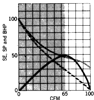
Fig 14-39. Characteristic curves for propeller fans
