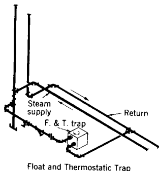
Fig 15-25. Supply riser drip connection
