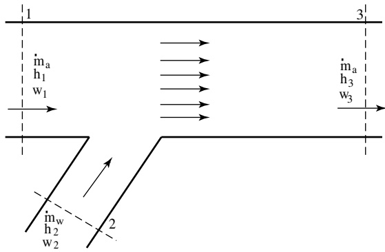
Fig 3-10. Adiabatic mixing of two streams process
