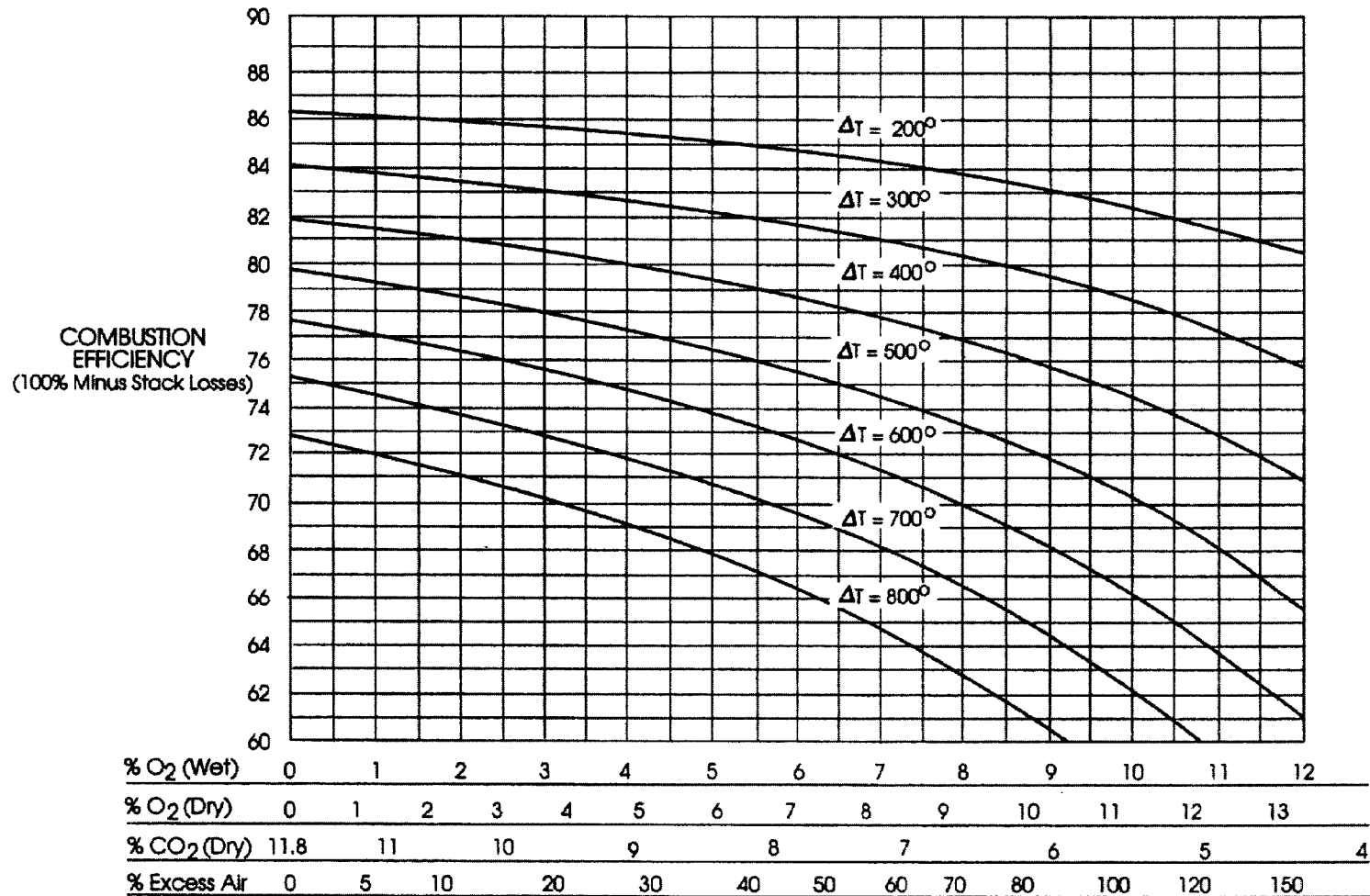
Fig 12-5. Combustion efficiency of natural gas
