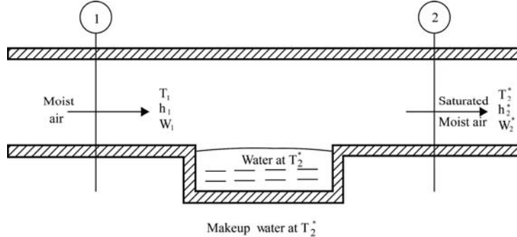
Fig 2-3. Adiabatic saturation of air
