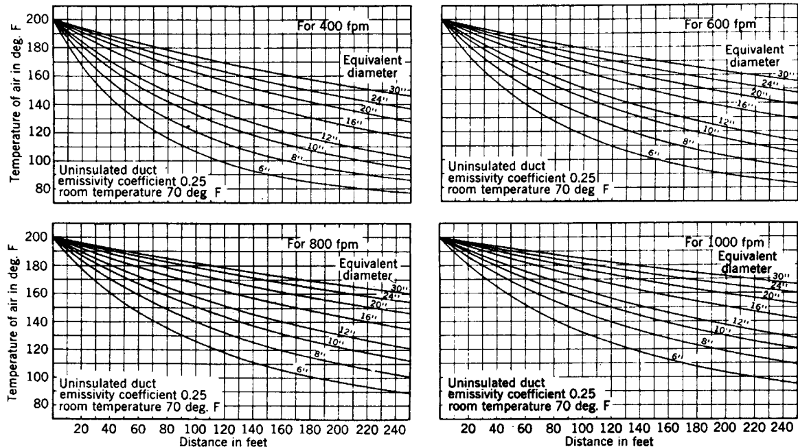
Fig 15-141. Temperature drop in ducts for different air velocity
