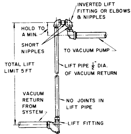
Fig 15-46. One step condensate lift
