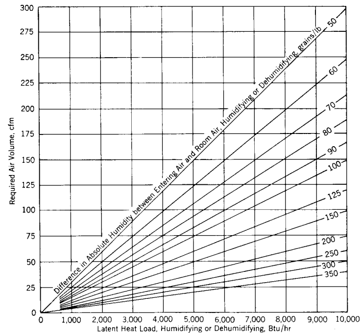
Fig 14-77. Air volume required to handle humidifying or dehumidifying loads
