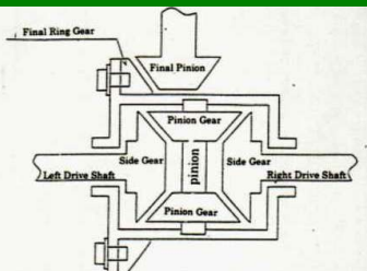
Differential gear
