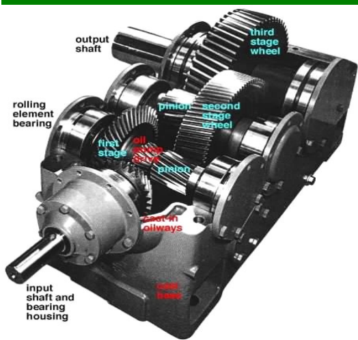
Gearbox
