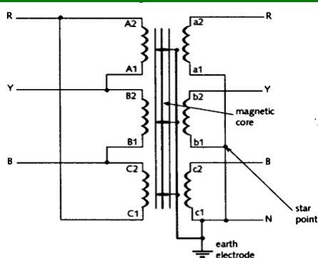
Delta-star transformer
