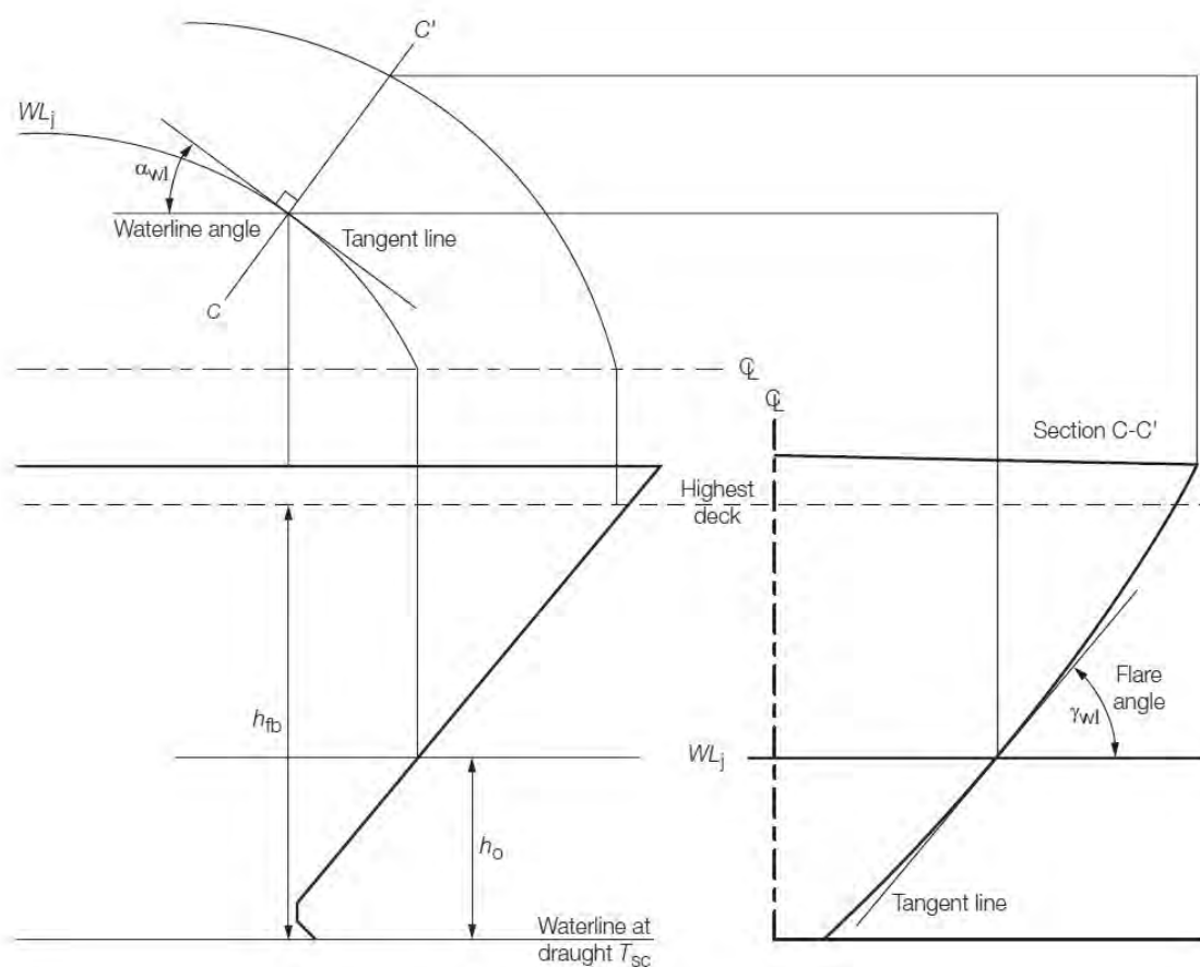
Figure 2.4.2 Definition of bow geometry
