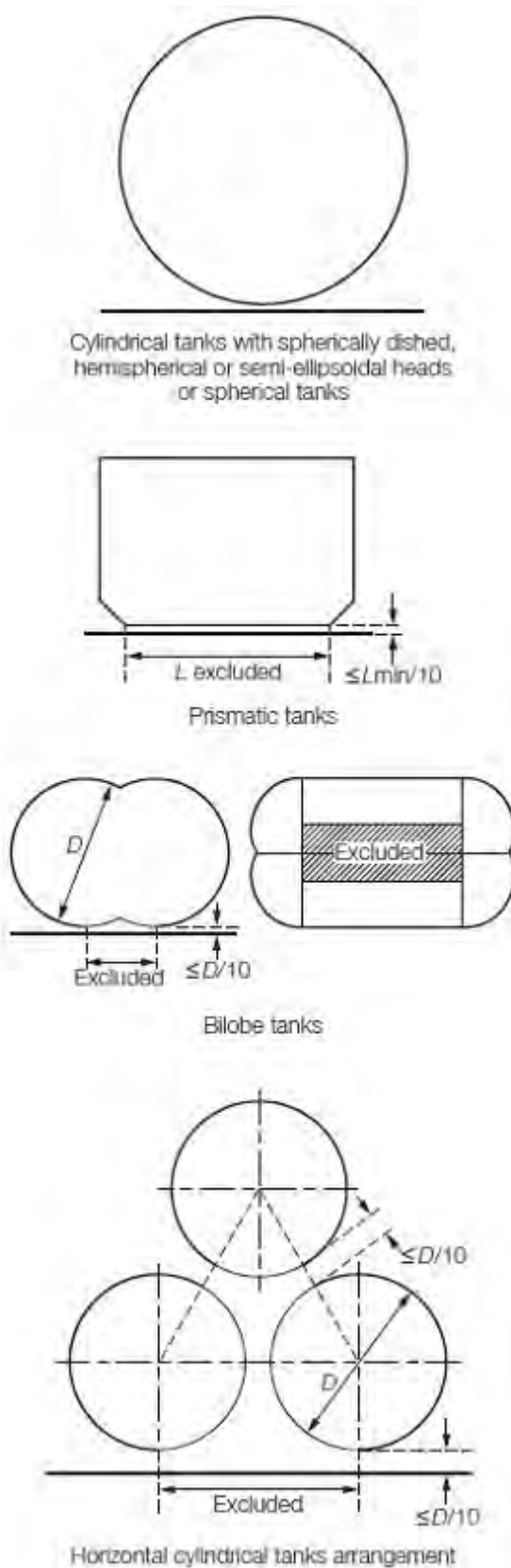
Figure 8.1.1 Horizontal cylindrical tanks arrangement
