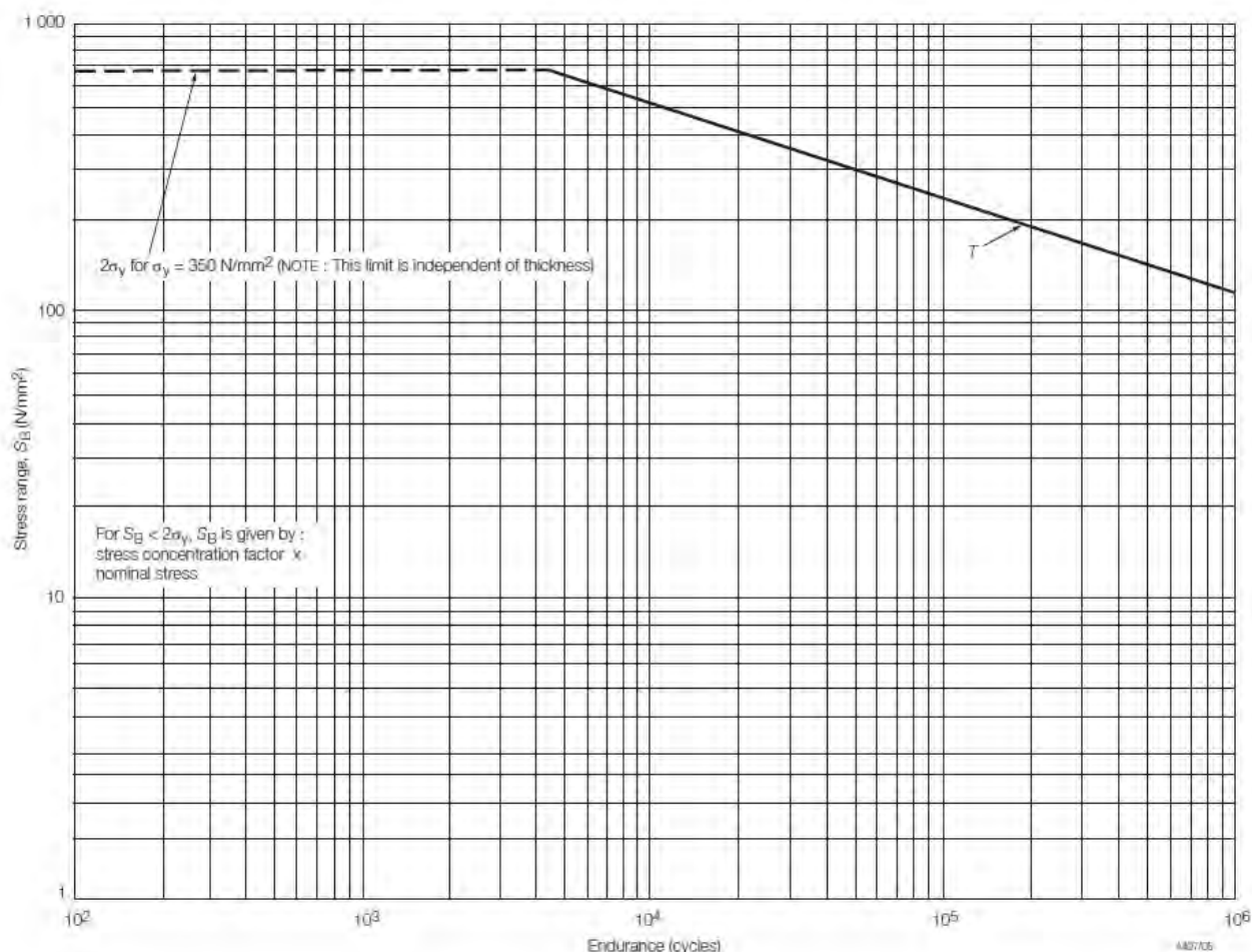
Figure 12.2.4 Treatment of high cyclic stresses for the T-curve and a material with yield stress = 350 N/mm 2
