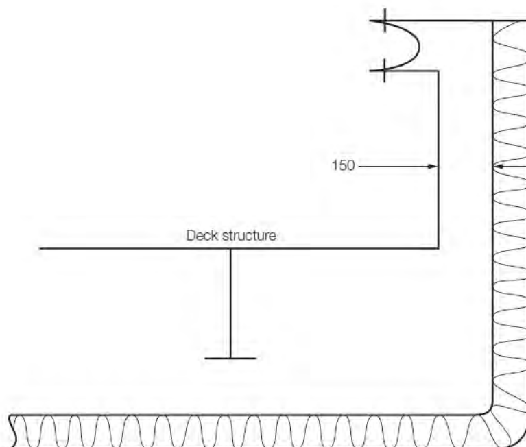
Figure 3.1.6 Minimum distance between cargo tank dome and deck structure
