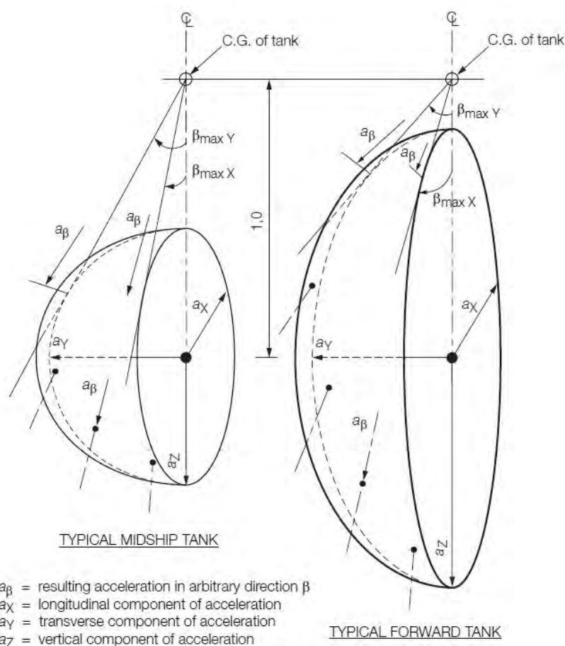
Figure 4.7.3 Acceleration ellipsoids
