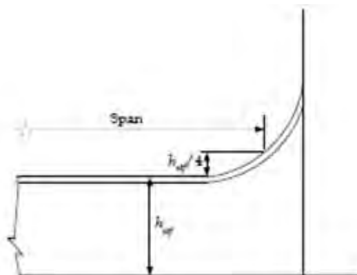
Figure 1.8.3 Effective Bending Span for Local Support Members with Continuous Face Plate along Bracket Edge
