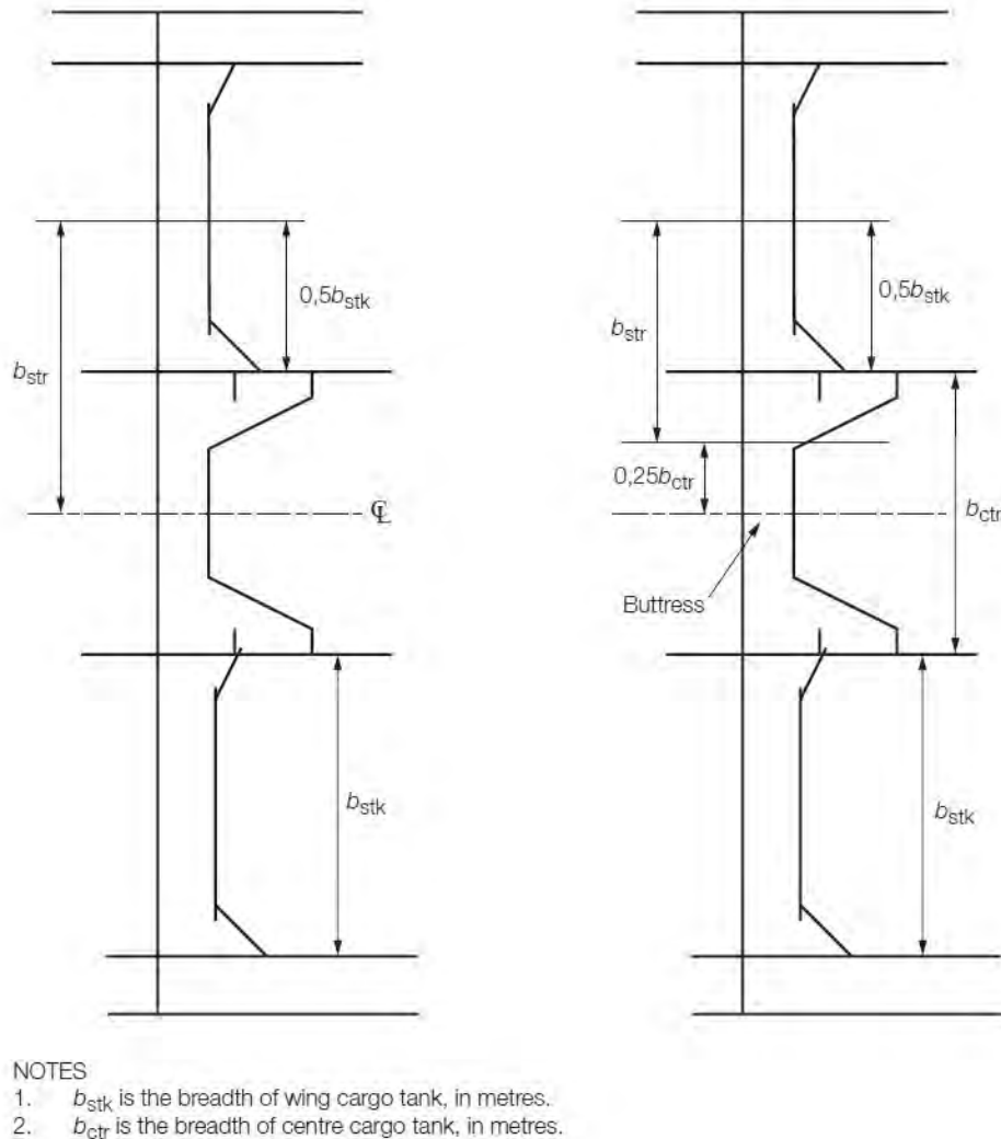
Figure 3.1.6 Load breadth of stringers for units with two inner longitudinal bulkheads
