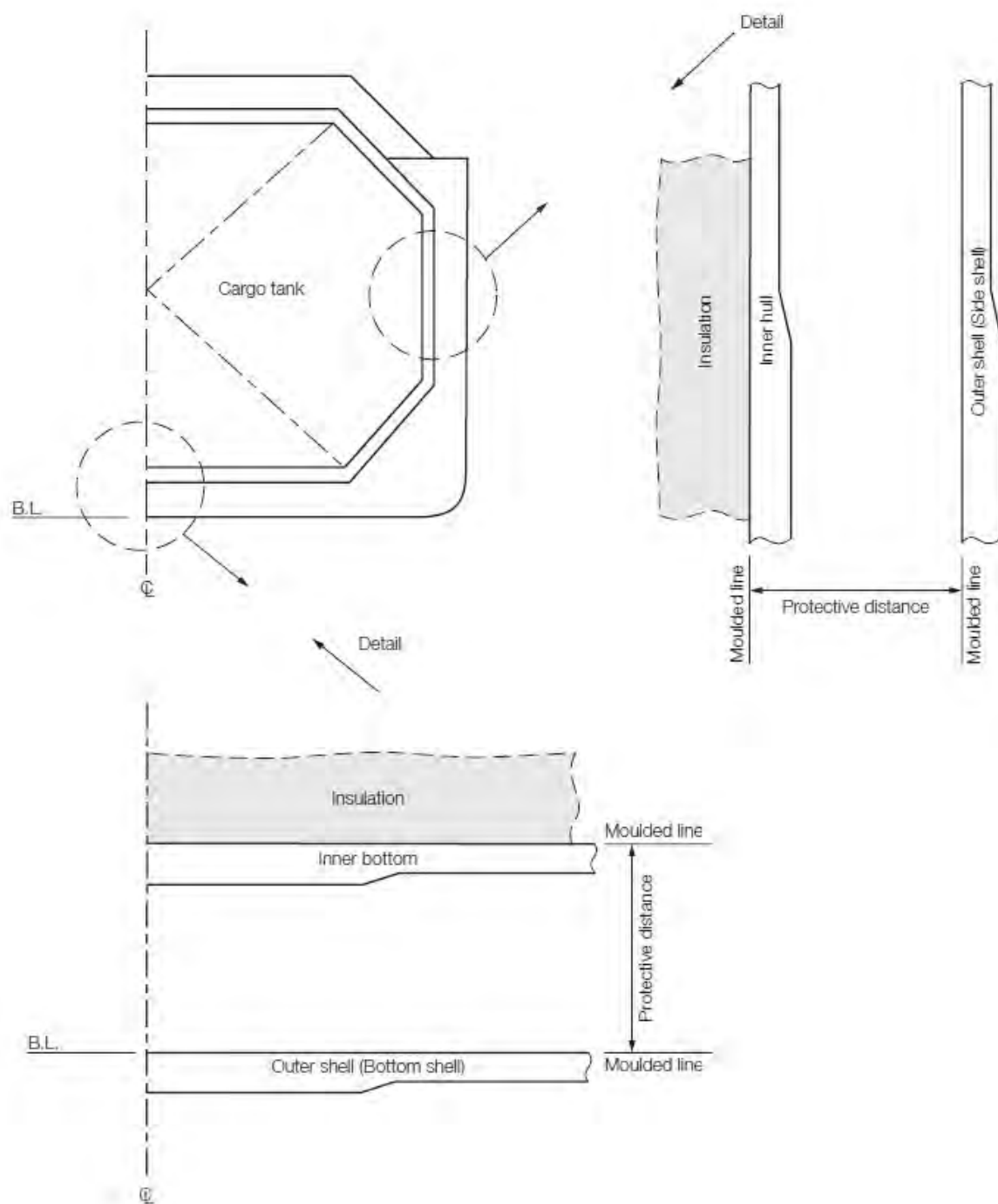
Figure 2.1.3 Membrane tank, protective distance
