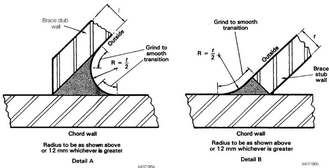
Figure 8.2.8 Weld grinding
