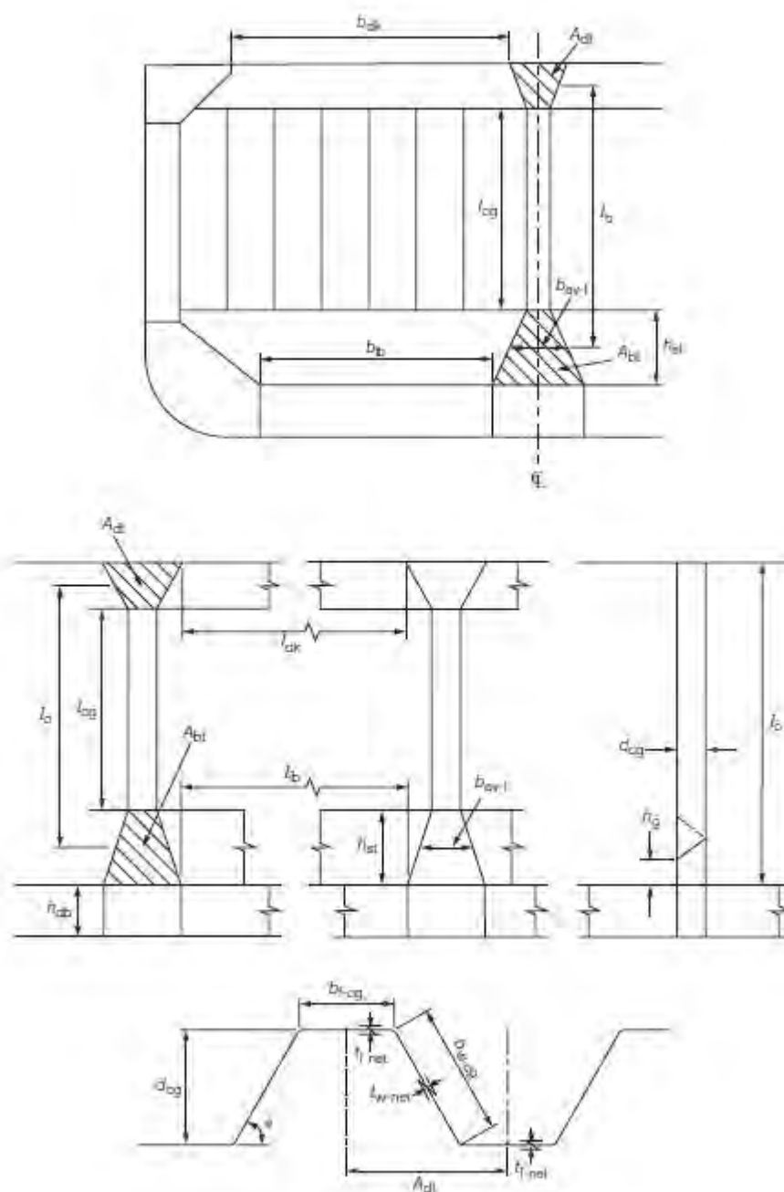
Figure 3.2.3 Definition of parameters for corrugated bulkhead (units with longitudinal bulkhead at centreline)
