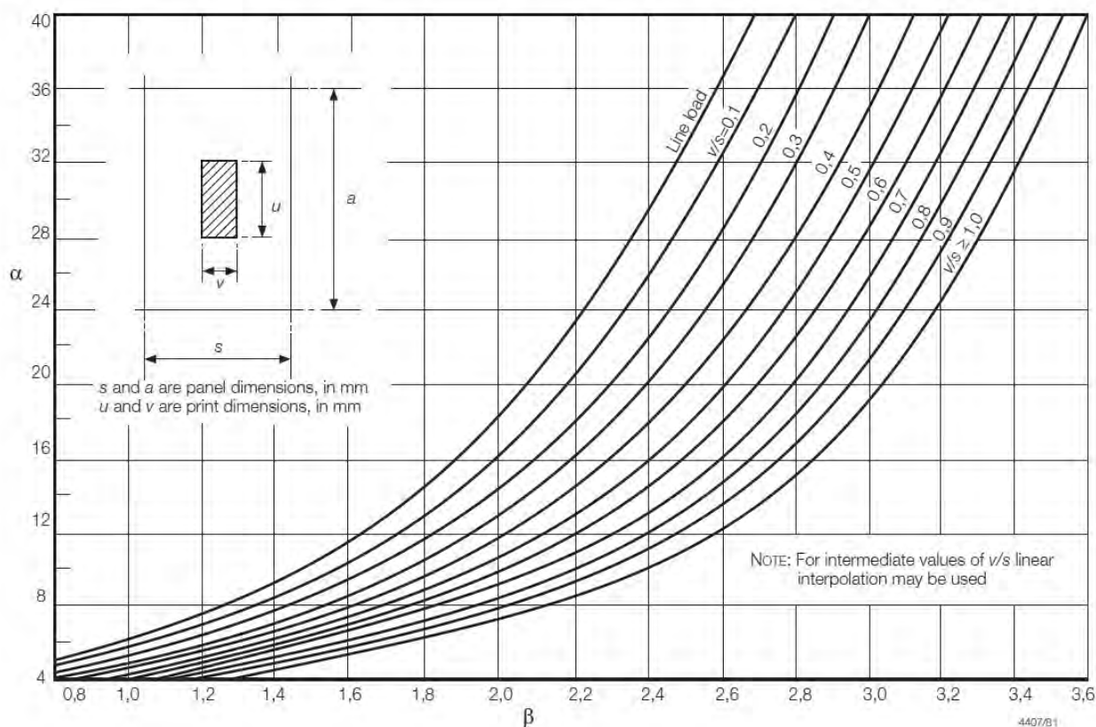
Figure 6.5.1 Tyre print chart
