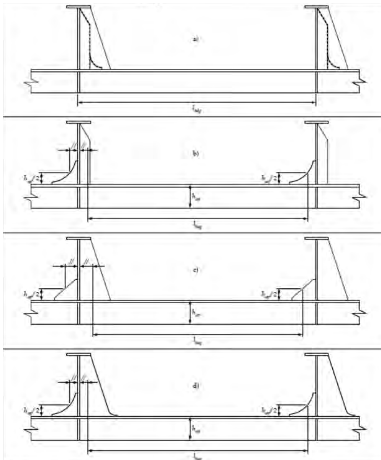
Figure 1.8.2 Effective Bending Span of Stiffeners Supported by Web Stiffeners (Single Skin Construction)
