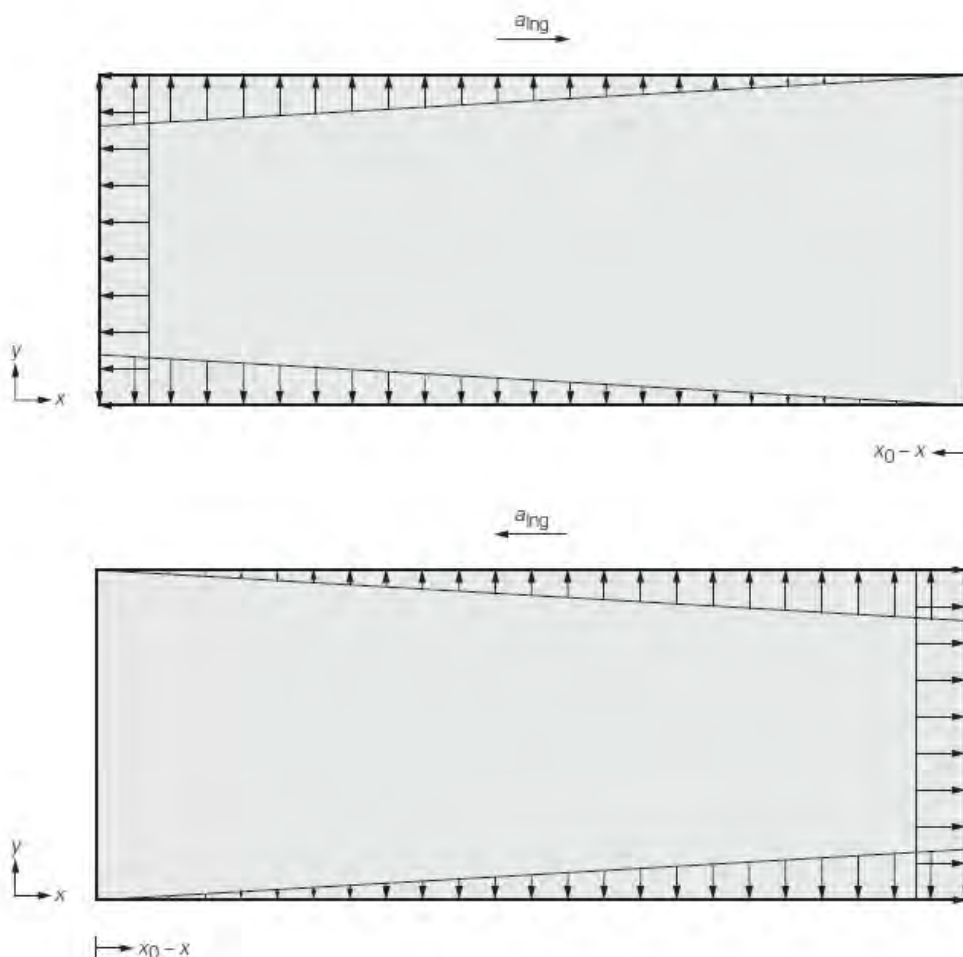
Figure 2.6.6 Dynamic tank pressure in tanks due to positive and negative longitudinal acceleration
