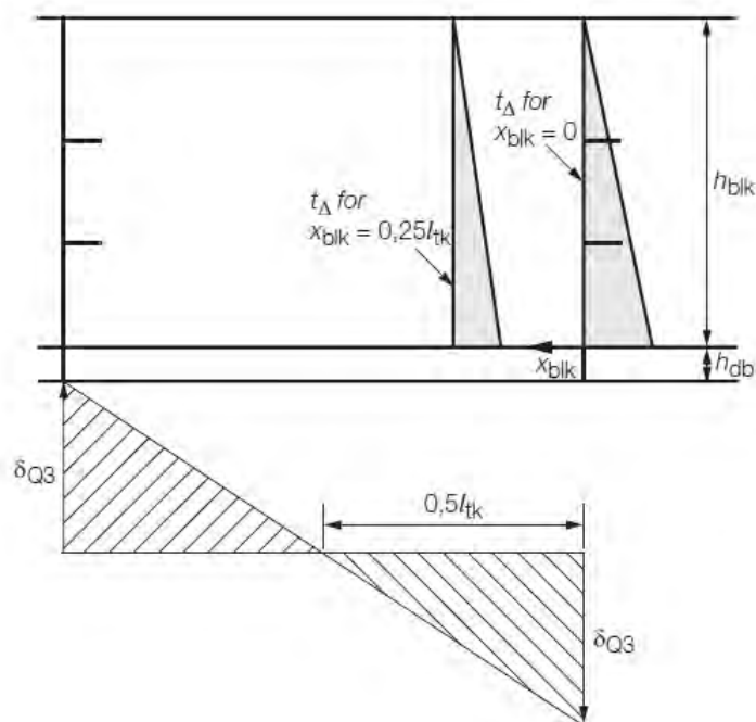
Figure 3.1.1 Shear force correction for longitudinal bulkheads
