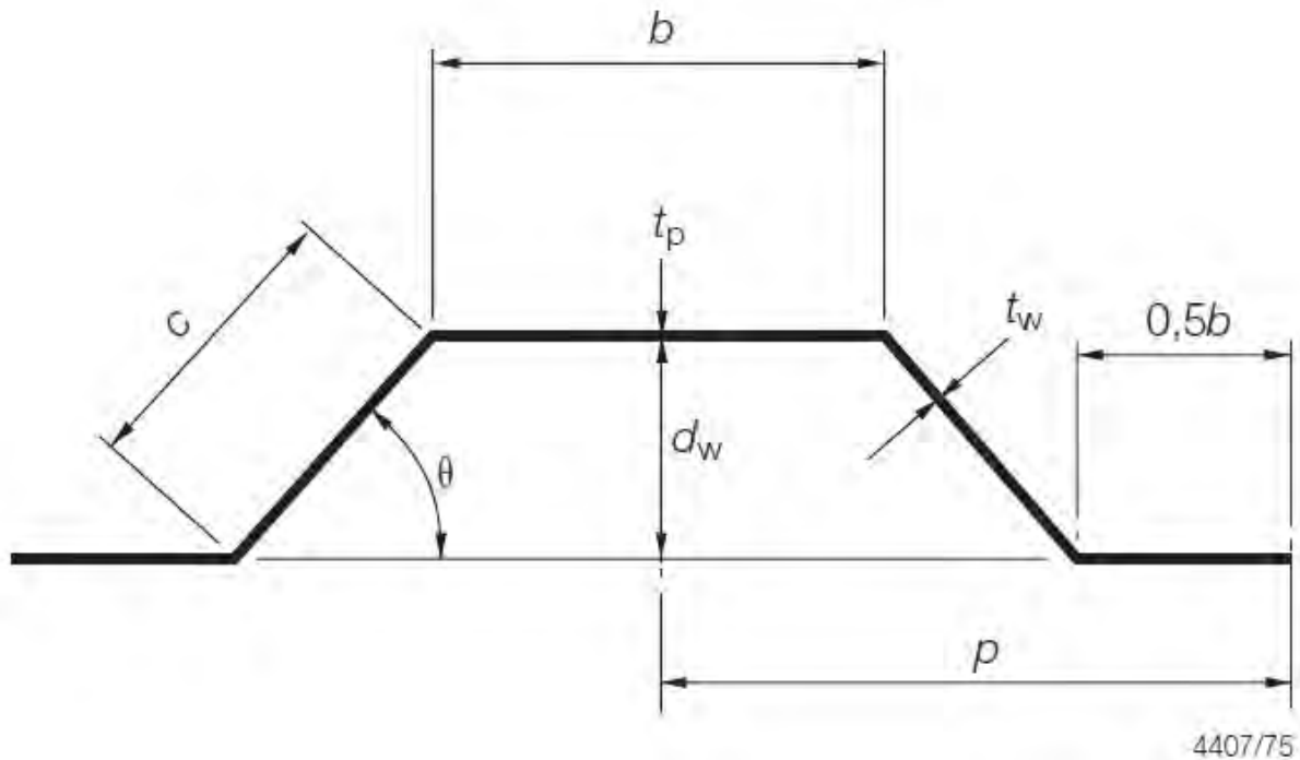
Figure 3.3.1 Corrugation geometry
