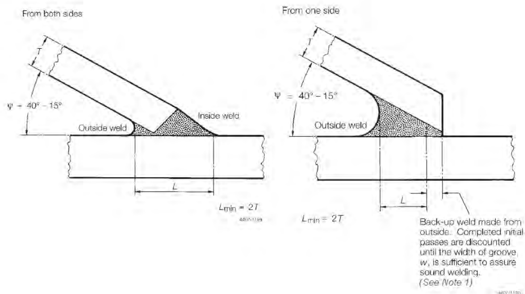
Figure 8.2.7 Welding at location 5
