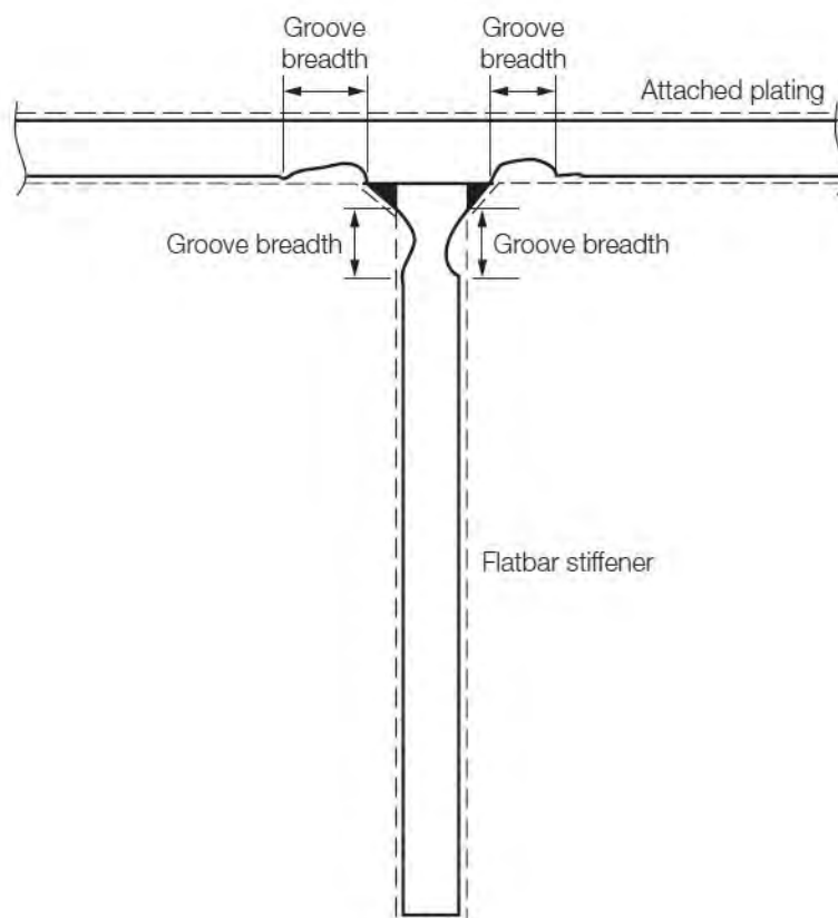
Figure 1.13.3 Groove corrosion
