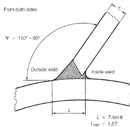
Figure 8.2.4 Welding at location 2
