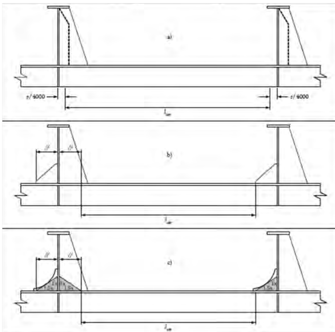
Figure 1.8.5 Effective Shear Span of Stiffeners Supported by Web Stiffeners (Single Skin Construction)
