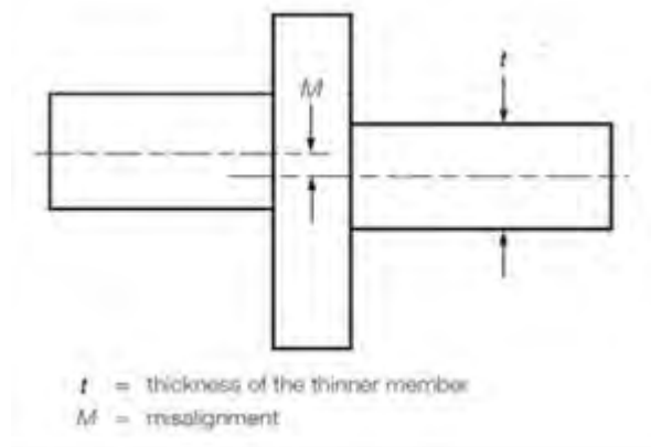
Figure 8.6.2 Misalignment of non-continuous plates
