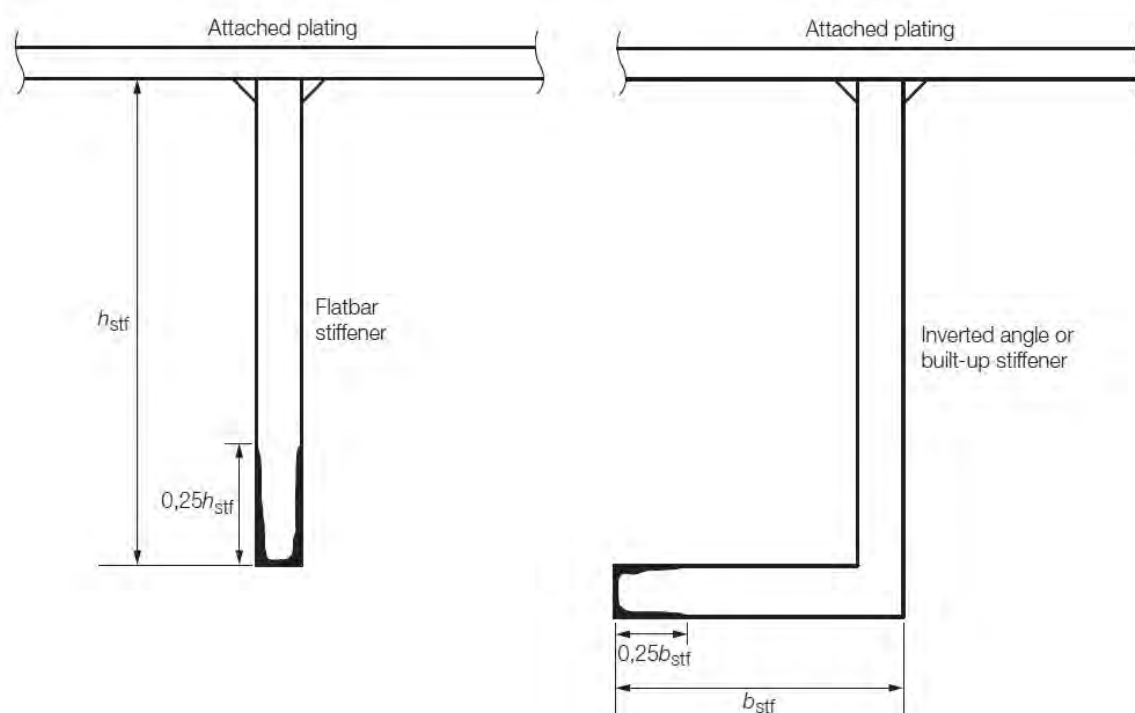
Figure 1.13.2 Edge corrosion
