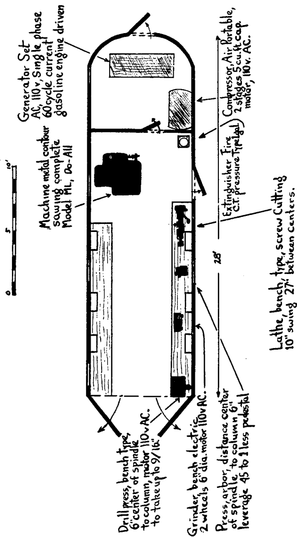
FIGURE 9.—Floor diagram of typical machine shop trailer.
